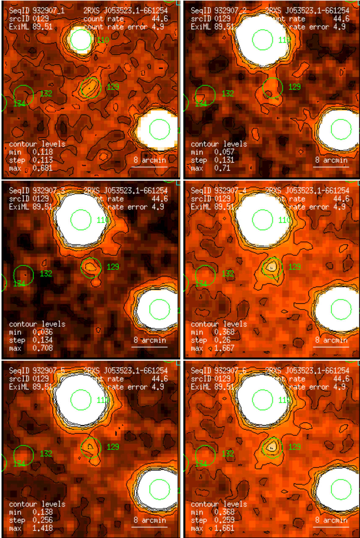
Figure 129: RASS 932907: detection 0129: band rate images, Gaussian filter: (1) PSPC channels 11 – 41, (2) 52 – 90, (3) 91 – 201, (4) 11 – 235, (5) 52 – 201, (6) 11 – 201. Broad band rates in counts/ks. Band rate contour levels in counts/ks/arcmin 2 .
