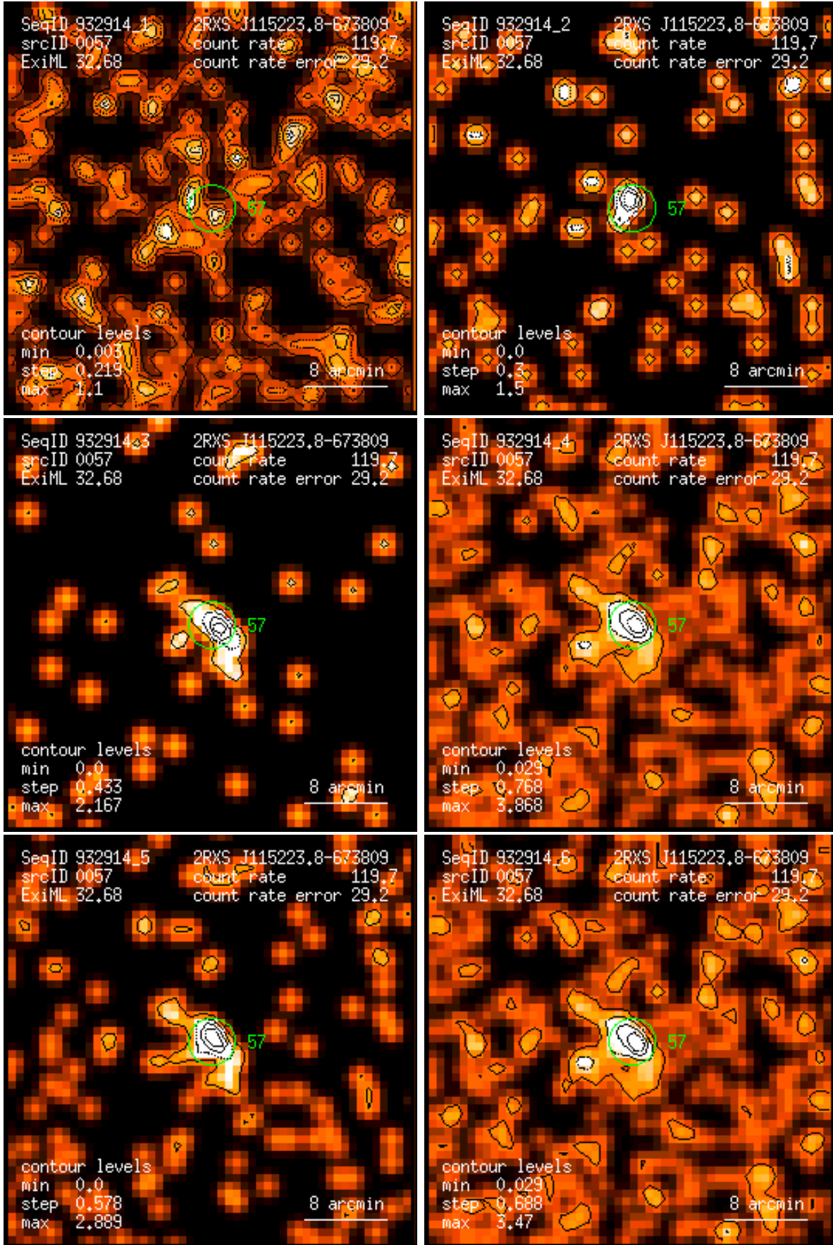
Figure 57: RASS 932914: detection 0057: band rate images, Gaussian filter: (1) PSPC channels 11 – 41, (2) 52 – 90, (3) 91 – 201, (4) 11 – 235, (5) 52 – 201, (6) 11 – 201. Broad band rates in counts/ks. Band rate contour levels in counts/ks/arcmin 2 .
