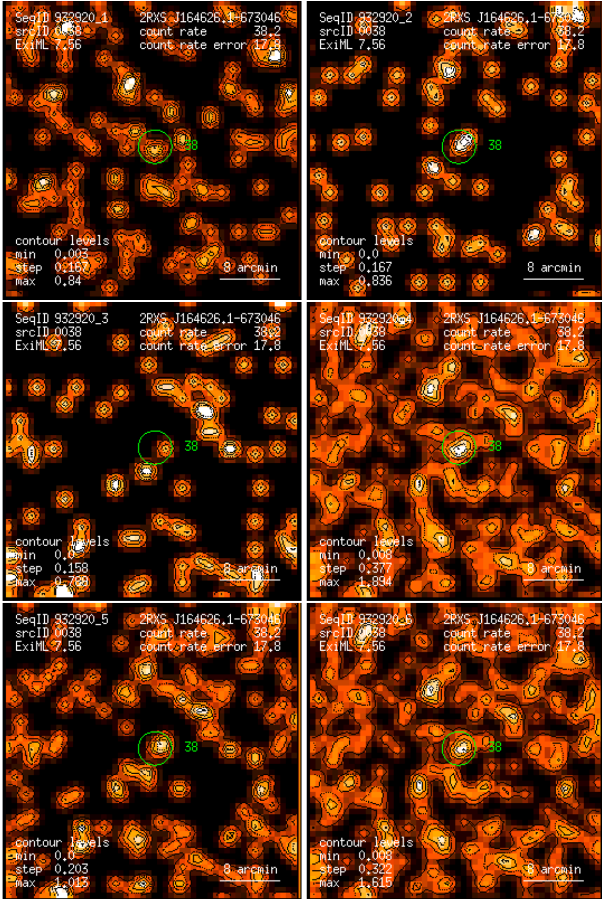
Figure 38: RASS 932920: detection 0038: band rate images, Gaussian filter: (1) PSPC channels 11 – 41, (2) 52 – 90, (3) 91 – 201, (4) 11 – 235, (5) 52 – 201, (6) 11 – 201. Broad band rates in counts/ks. Band rate contour levels in counts/ks/arcmin 2 .
