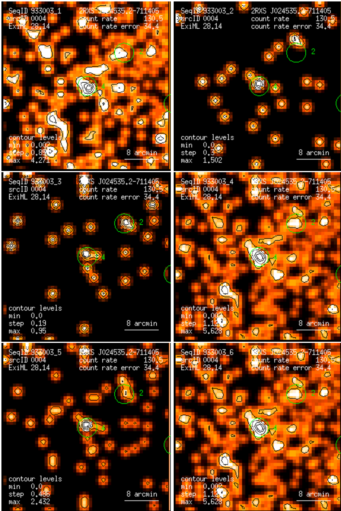
Figure 4: RASS 933003: detection 0004: band rate images, Gaussian filter: (1) PSPC channels 11 – 41, (2) 52 – 90, (3) 91 – 201, (4) 11 – 235, (5) 52 – 201, (6) 11 – 201. Broad band rates in counts/ks. Band rate contour levels in counts/ks/arcmin 2 .
