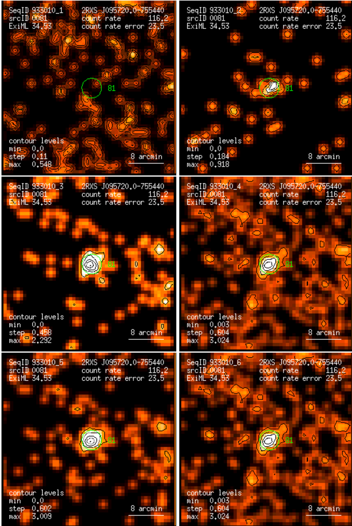
Figure 81: RASS 933010: detection 0081: band rate images, Gaussian filter: (1) PSPC channels 11 – 41, (2) 52 – 90, (3) 91 – 201, (4) 11 – 235, (5) 52 – 201, (6) 11 – 201. Broad band rates in counts/ks. Band rate contour levels in counts/ks/arcmin 2 .
