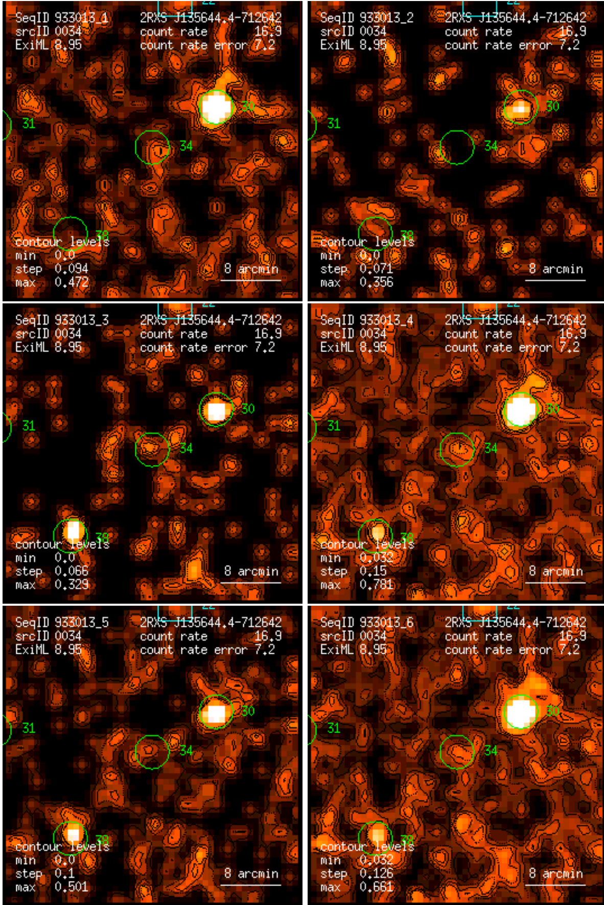
Figure 34: RASS 933013: detection 0034: band rate images, Gaussian filter: (1) PSPC channels 11 – 41, (2) 52 – 90, (3) 91 – 201, (4) 11 – 235, (5) 52 – 201, (6) 11 – 201. Broad band rates in counts/ks. Band rate contour levels in counts/ks/arcmin 2 .
