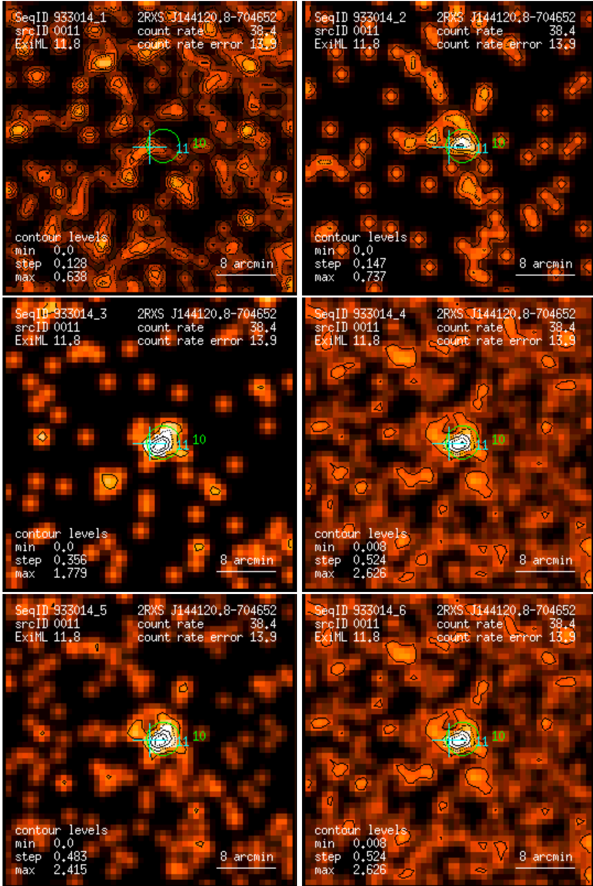
Figure 11: RASS 933014: detection 0011: band rate images, Gaussian filter: (1) PSPC channels 11 – 41, (2) 52 – 90, (3) 91 – 201, (4) 11 – 235, (5) 52 – 201, (6) 11 – 201. Broad band rates in counts/ks. Band rate contour levels in counts/ks/arcmin 2 .
