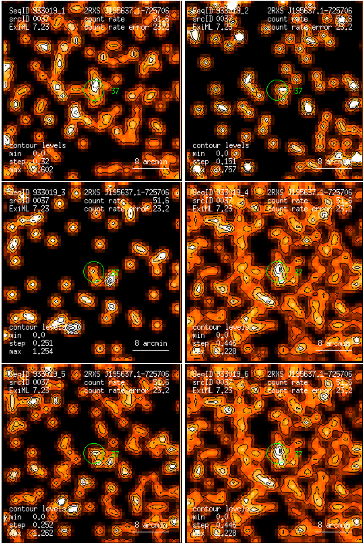
Figure 37: RASS 933019: detection 0037: band rate images, Gaussian filter: (1) PSPC channels 11 – 41, (2) 52 – 90, (3) 91 – 201, (4) 11 – 235, (5) 52 – 201, (6) 11 – 201. Broad band rates in counts/ks. Band rate contour levels in counts/ks/arcmin 2 .
