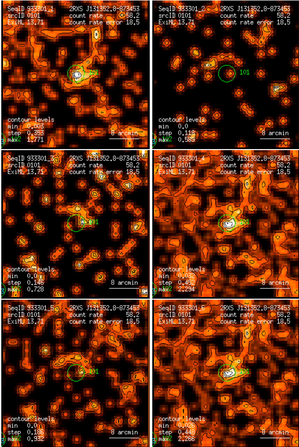
Figure 101: RASS 933301: detection 0101: band rate images, Gaussian filter: (1) PSPC channels 11 – 41, (2) 52 – 90, (3) 91 – 201, (4) 11 – 235, (5) 52 – 201, (6) 11 – 201. Broad band rates in counts/ks. Band rate contour levels in counts/ks/arcmin 2 .
