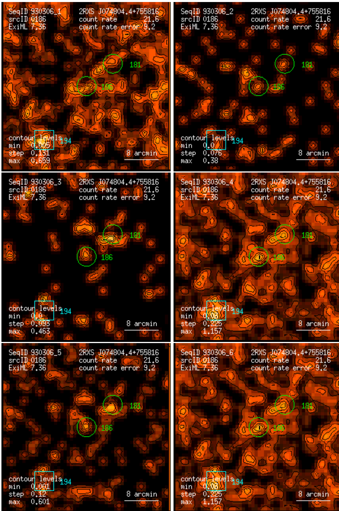
Figure 186: RASS 930306: detection 0186: band rate images, Gaussian filter: (1) PSPC channels 11 – 41, (2) 52 – 90, (3) 91 – 201, (4) 11 – 235, (5) 52 – 201, (6) 11 – 201. Broad band rates in counts/ks. Band rate contour levels in counts/ks/arcmin 2 .
