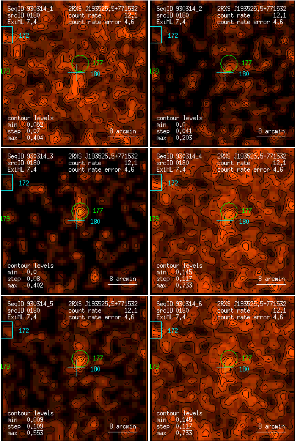
Figure 180: RASS 930314: detection 0180: band rate images, Gaussian filter: (1) PSPC channels 11 – 41, (2) 52 – 90, (3) 91 – 201, (4) 11 – 235, (5) 52 – 201, (6) 11 – 201. Broad band rates in counts/ks. Band rate contour levels in counts/ks/arcmin 2 .
