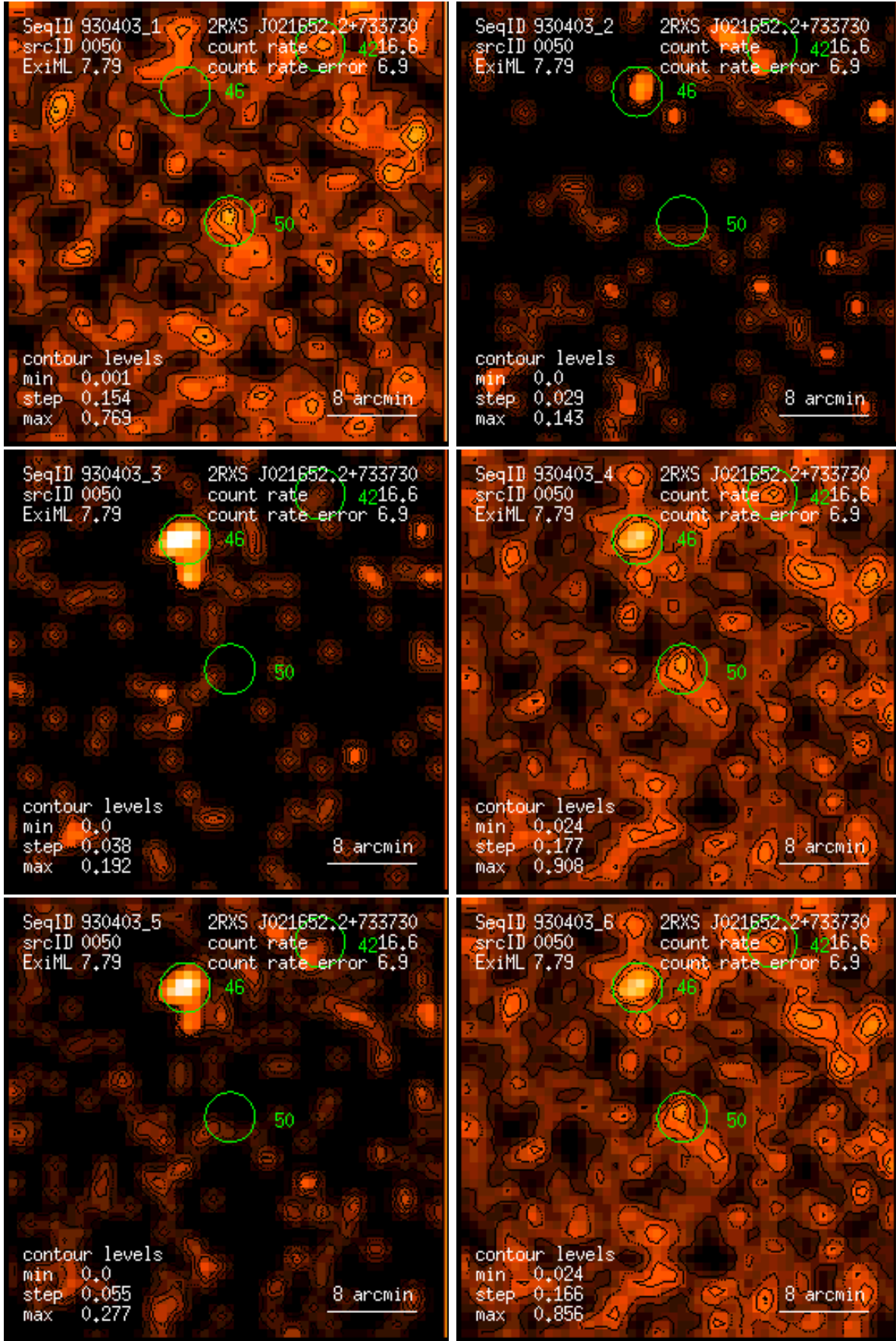
Figure 50: RASS 930403: detection 0050: band rate images, Gaussian filter: (1) PSPC channels 11 – 41, (2) 52 – 90, (3) 91 – 201, (4) 11 – 235, (5) 52 – 201, (6) 11 – 201. Broad band rates in counts/ks. Band rate contour levels in counts/ks/arcmin 2 .
