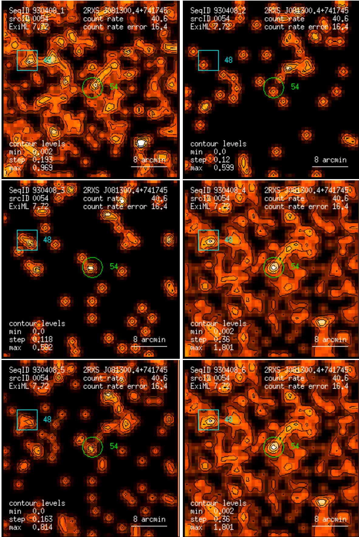
Figure 54: RASS 930408: detection 0054: band rate images, Gaussian filter: (1) PSPC channels 11 – 41, (2) 52 – 90, (3) 91 – 201, (4) 11 – 235, (5) 52 – 201, (6) 11 – 201. Broad band rates in counts/ks. Band rate contour levels in counts/ks/arcmin 2 .
