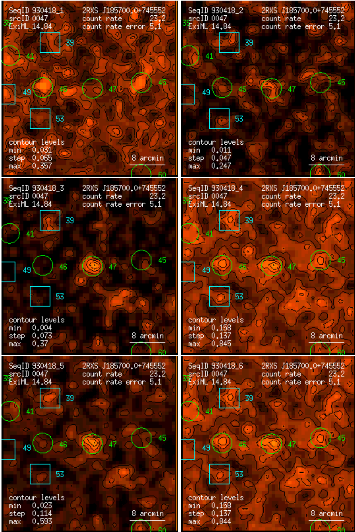
Figure 47: RASS 930418: detection 0047: band rate images, Gaussian filter: (1) PSPC channels 11 – 41, (2) 52 – 90, (3) 91 – 201, (4) 11 – 235, (5) 52 – 201, (6) 11 – 201. Broad band rates in counts/ks. Band rate contour levels in counts/ks/arcmin 2 .
