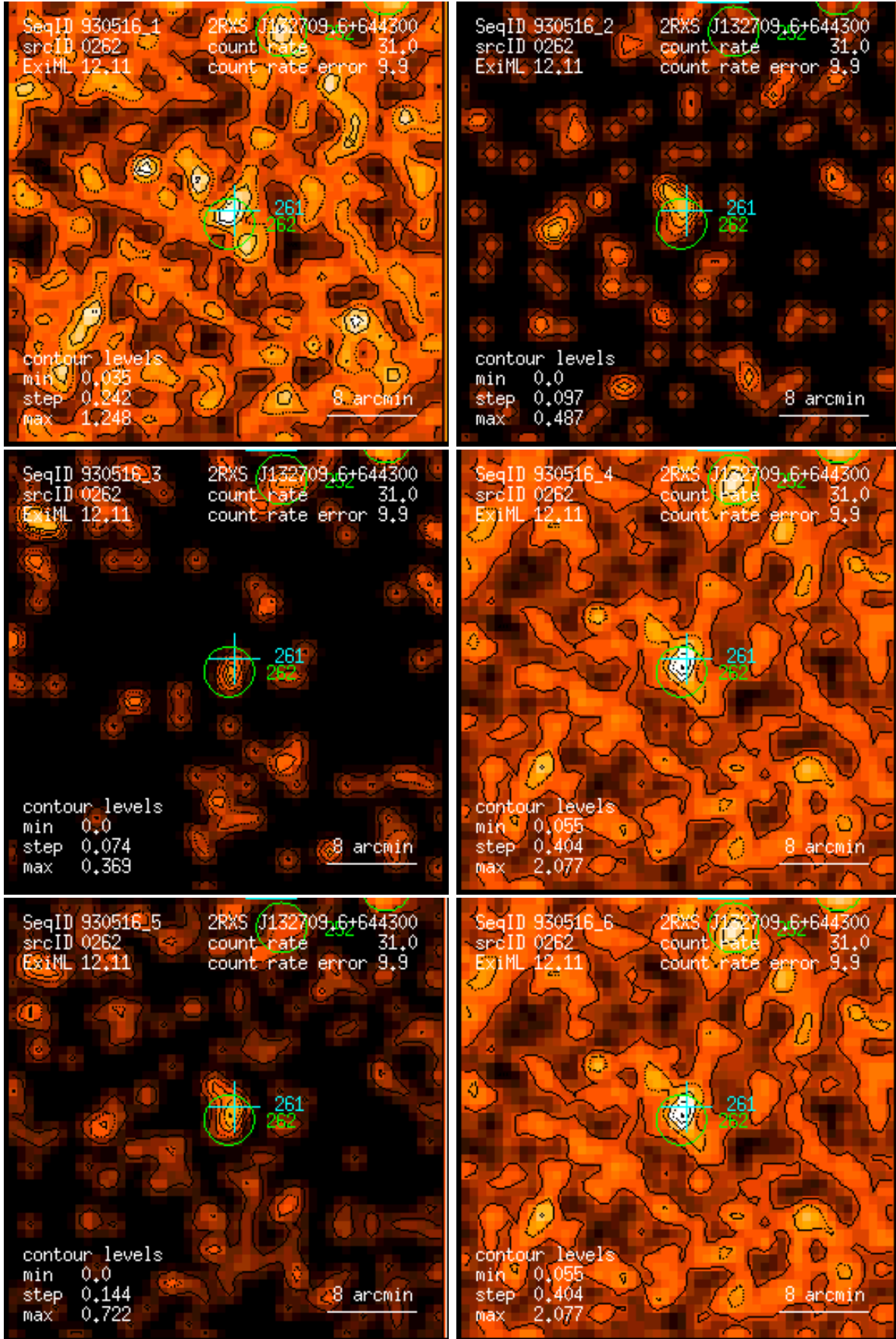
Figure 262: RASS 930516: detection 0262: band rate images, Gaussian filter: (1) PSPC channels 11 – 41, (2) 52 – 90, (3) 91 – 201, (4) 11 – 235, (5) 52 – 201, (6) 11 – 201. Broad band rates in counts/ks. Band rate contour levels in counts/ks/arcmin 2 .
