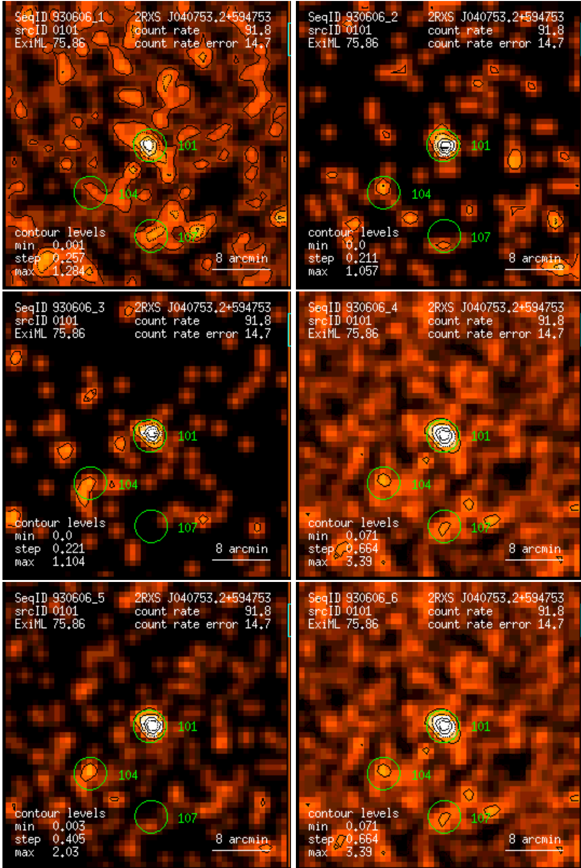
Figure 101: RASS 930606: detection 0101: band rate images, Gaussian filter: (1) PSPC channels 11 – 41, (2) 52 – 90, (3) 91 – 201, (4) 11 – 235, (5) 52 – 201, (6) 11 – 201. Broad band rates in counts/ks. Band rate contour levels in counts/ks/arcmin 2 .
