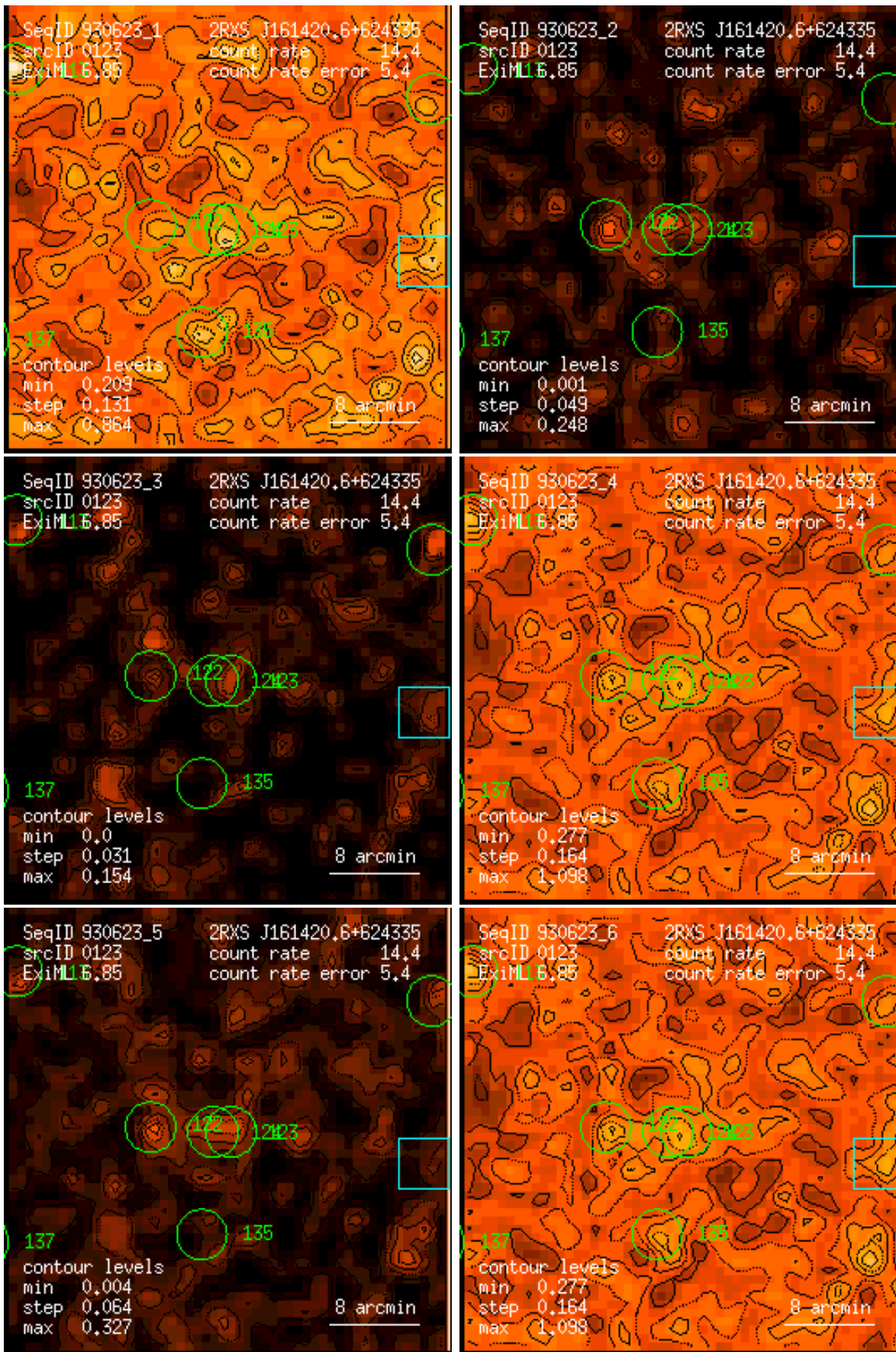
Figure 123: RASS 930623: detection 0123: band rate images, Gaussian filter: (1) PSPC channels 11 – 41, (2) 52 – 90, (3) 91 – 201, (4) 11 – 235, (5) 52 – 201, (6) 11 – 201. Broad band rates in counts/ks. Band rate contour levels in counts/ks/arcmin 2 .
