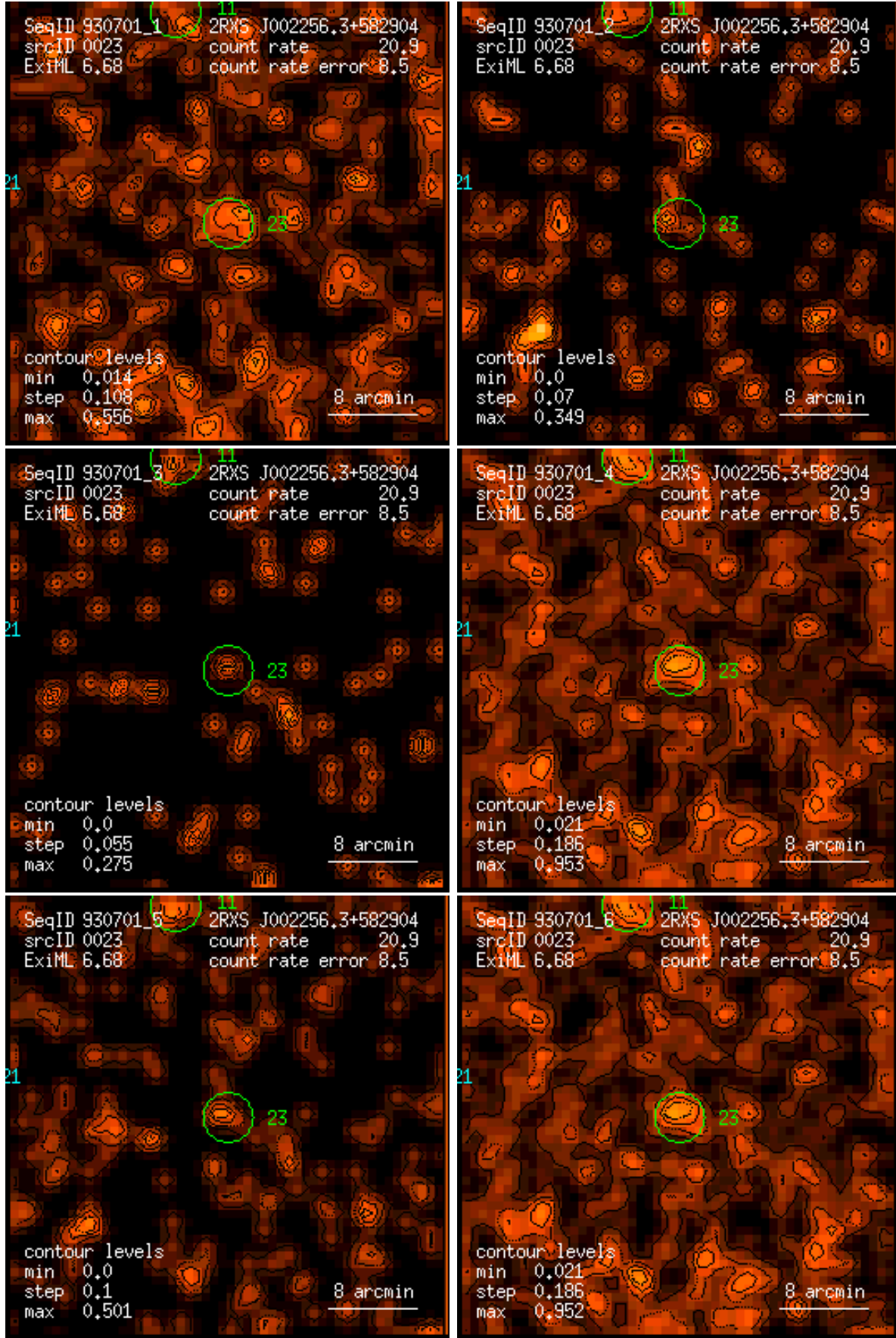
Figure 23: RASS 930701: detection 0023: band rate images, Gaussian filter: (1) PSPC channels 11 – 41, (2) 52 – 90, (3) 91 – 201, (4) 11 – 235, (5) 52 – 201, (6) 11 – 201. Broad band rates in counts/ks. Band rate contour levels in counts/ks/arcmin 2 .
