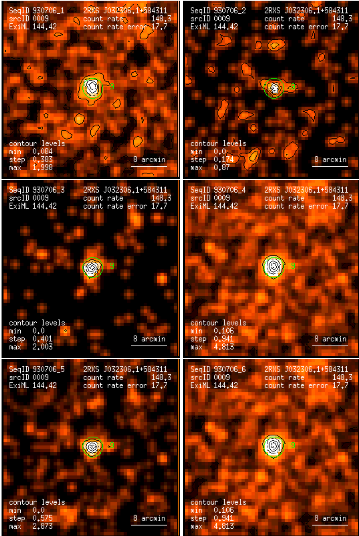
Figure 9: RASS 930706: detection 0009: band rate images, Gaussian filter: (1) PSPC channels 11 – 41, (2) 52 – 90, (3) 91 – 201, (4) 11 – 235, (5) 52 – 201, (6) 11 – 201. Broad band rates in counts/ks. Band rate contour levels in counts/ks/arcmin 2 .
