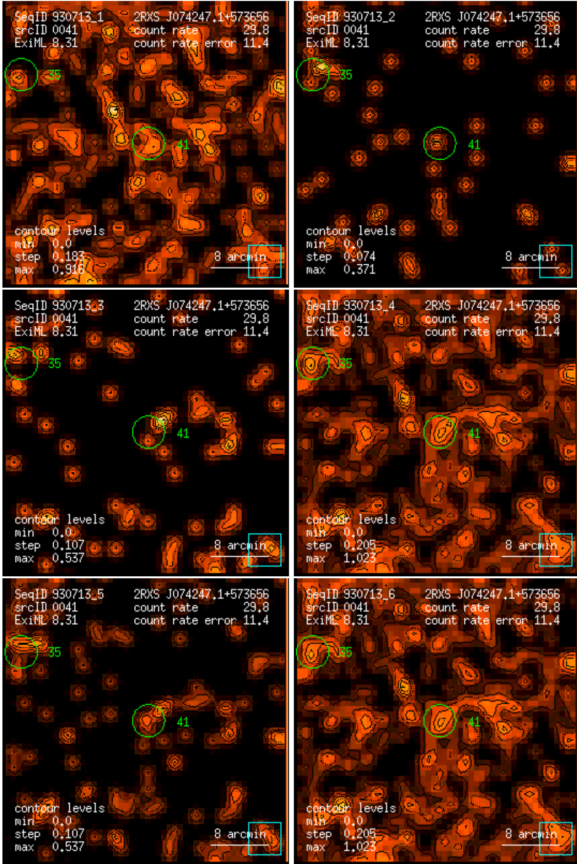
Figure 41: RASS 930713: detection 0041: band rate images, Gaussian filter: (1) PSPC channels 11 – 41, (2) 52 – 90, (3) 91 – 201, (4) 11 – 235, (5) 52 – 201, (6) 11 – 201. Broad band rates in counts/ks. Band rate contour levels in counts/ks/arcmin 2 .
