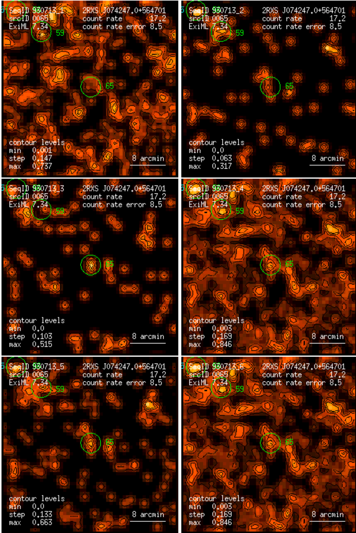
Figure 65: RASS 930713: detection 0065: band rate images, Gaussian filter: (1) PSPC channels 11 – 41, (2) 52 – 90, (3) 91 – 201, (4) 11 – 235, (5) 52 – 201, (6) 11 – 201. Broad band rates in counts/ks. Band rate contour levels in counts/ks/arcmin 2 .
