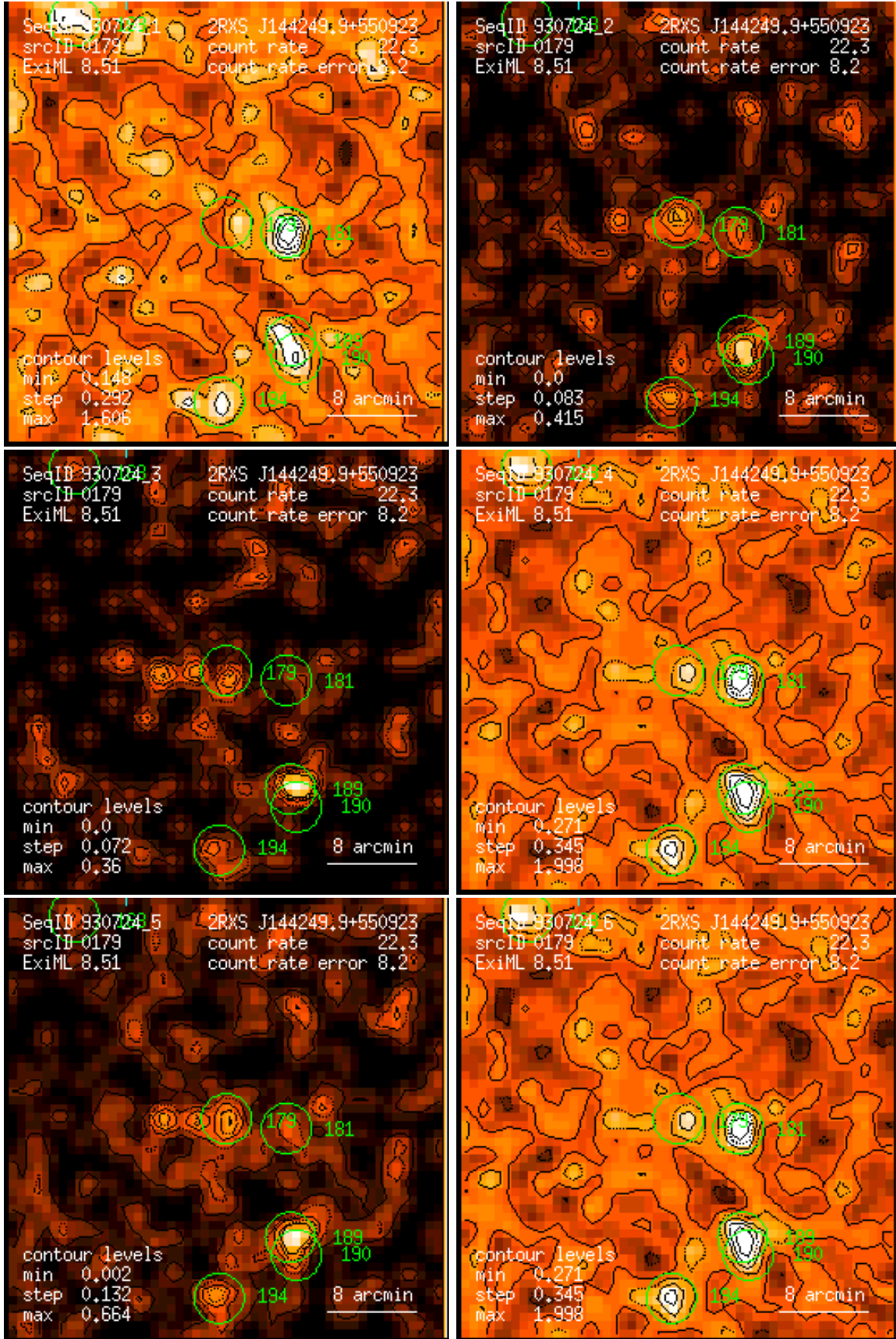
Figure 179: RASS 930724: detection 0179: band rate images, Gaussian filter: (1) PSPC channels 11 – 41, (2) 52 – 90, (3) 91 – 201, (4) 11 – 235, (5) 52 – 201, (6) 11 – 201. Broad band rates in counts/ks. Band rate contour levels in counts/ks/arcmin 2 .
