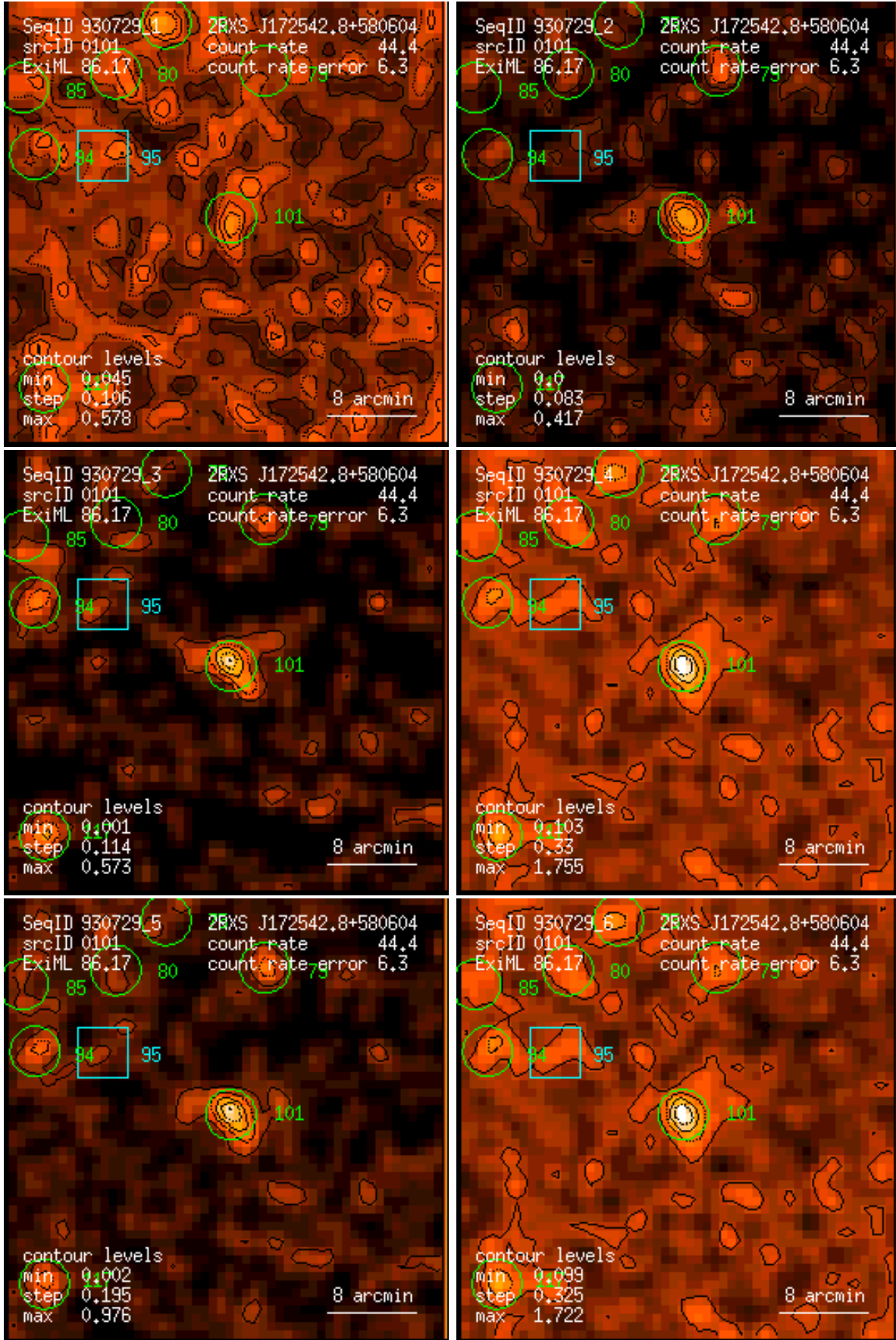
Figure 101: RASS 930729: detection 0101: band rate images, Gaussian filter: (1) PSPC channels 11 – 41, (2) 52 – 90, (3) 91 – 201, (4) 11 – 235, (5) 52 – 201, (6) 11 – 201. Broad band rates in counts/ks. Band rate contour levels in counts/ks/arcmin 2 .
