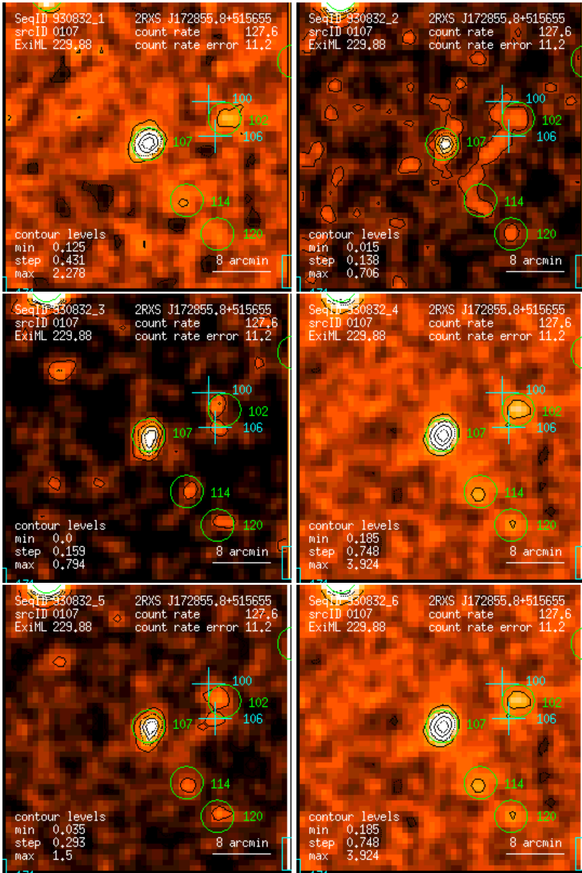
Figure 107: RASS 930832: detection 0107: band rate images, Gaussian filter: (1) PSPC channels 11 – 41, (2) 52 – 90, (3) 91 – 201, (4) 11 – 235, (5) 52 – 201, (6) 11 – 201. Broad band rates in counts/ks. Band rate contour levels in counts/ks/arcmin 2 .
