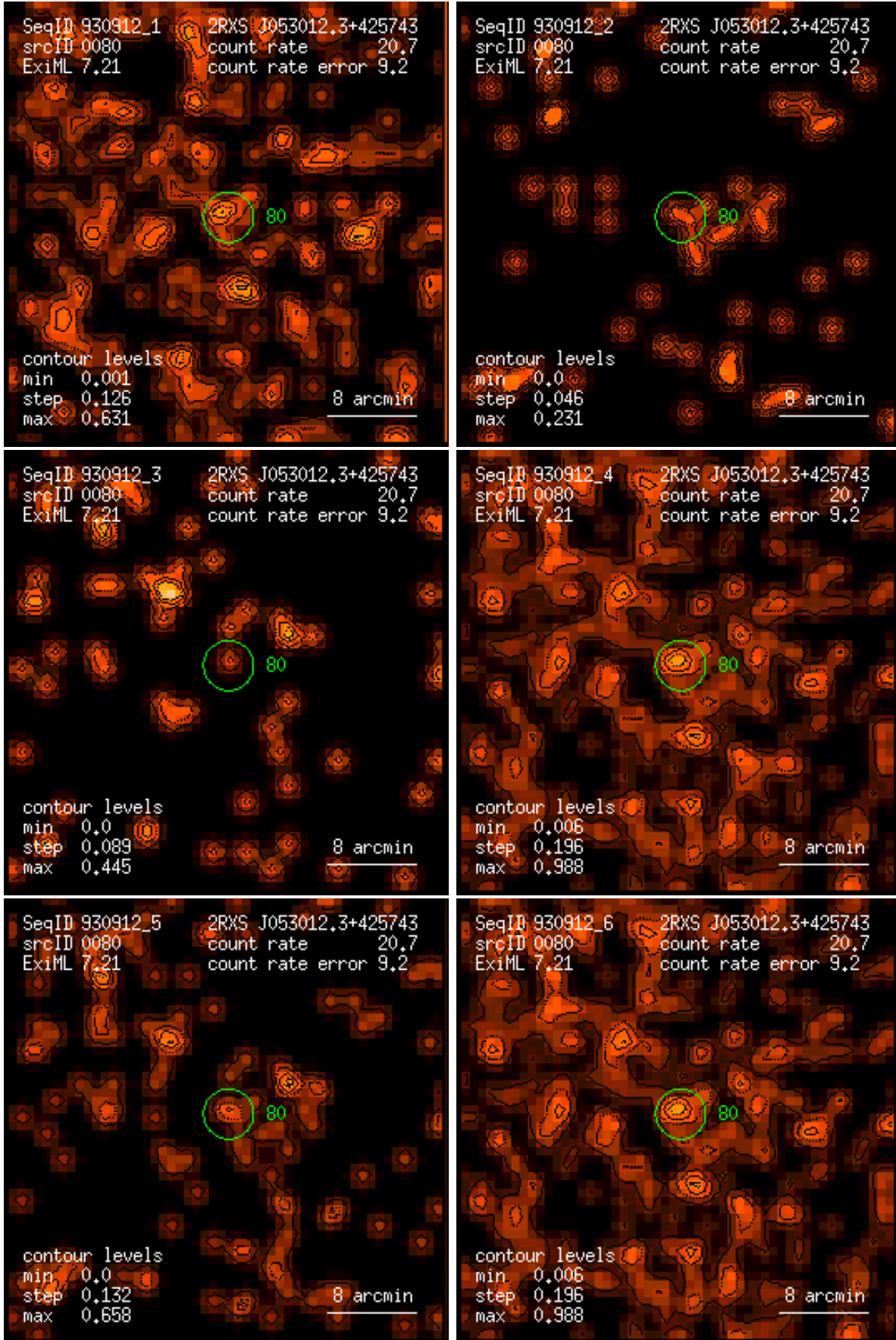
Figure 80: RASS 930912: detection 0080: band rate images, Gaussian filter: (1) PSPC channels 11 – 41, (2) 52 – 90, (3) 91 – 201, (4) 11 – 235, (5) 52 – 201, (6) 11 – 201. Broad band rates in counts/ks. Band rate contour levels in counts/ks/arcmin 2 .
