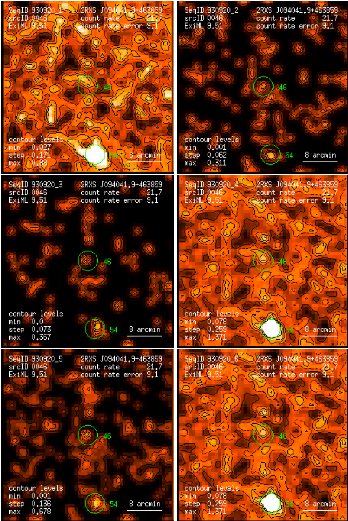
Figure 46: RASS 930920: detection 0046: band rate images, Gaussian filter: (1) PSPC channels 11 – 41, (2) 52 – 90, (3) 91 – 201, (4) 11 – 235, (5) 52 – 201, (6) 11 – 201. Broad band rates in counts/ks. Band rate contour levels in counts/ks/arcmin 2 .
