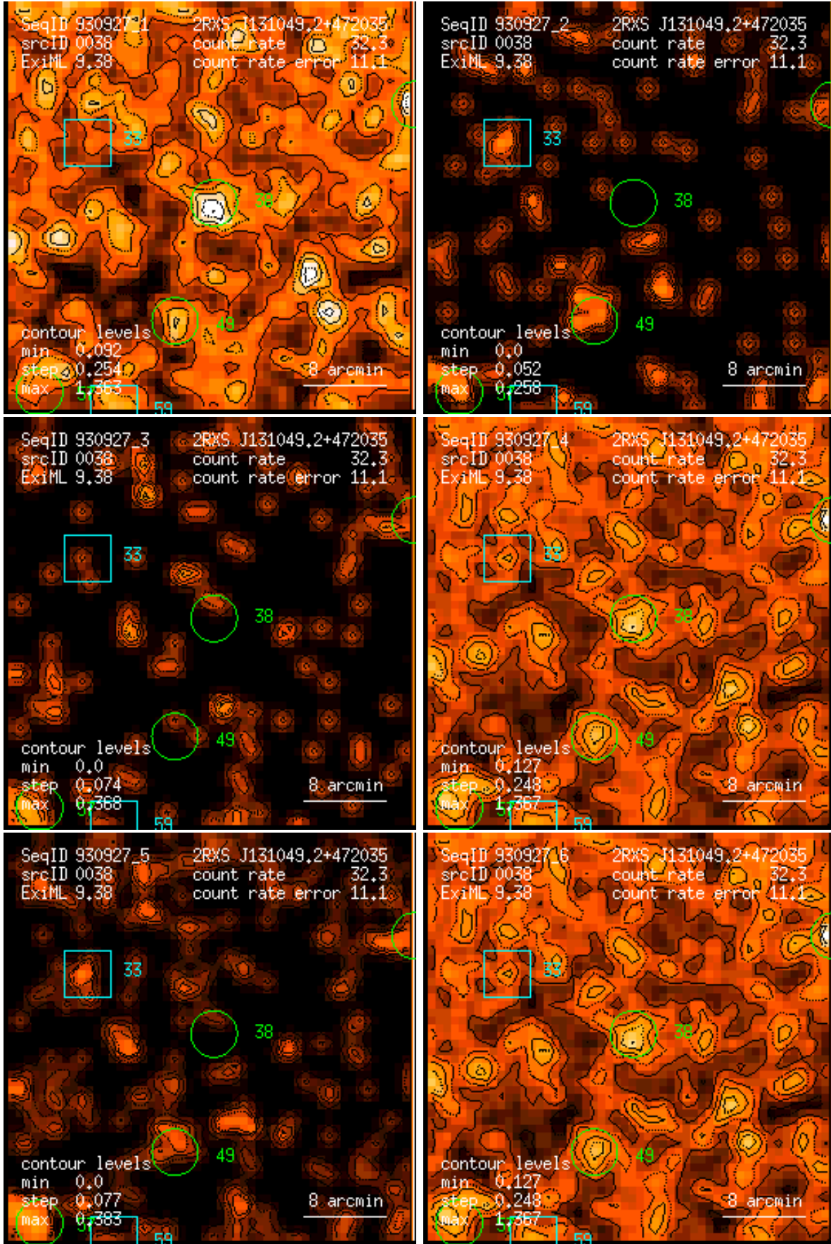
Figure 38: RASS 930927: detection 0038: band rate images, Gaussian filter: (1) PSPC channels 11 – 41, (2) 52 – 90, (3) 91 – 201, (4) 11 – 235, (5) 52 – 201, (6) 11 – 201. Broad band rates in counts/ks. Band rate contour levels in counts/ks/arcmin 2 .
