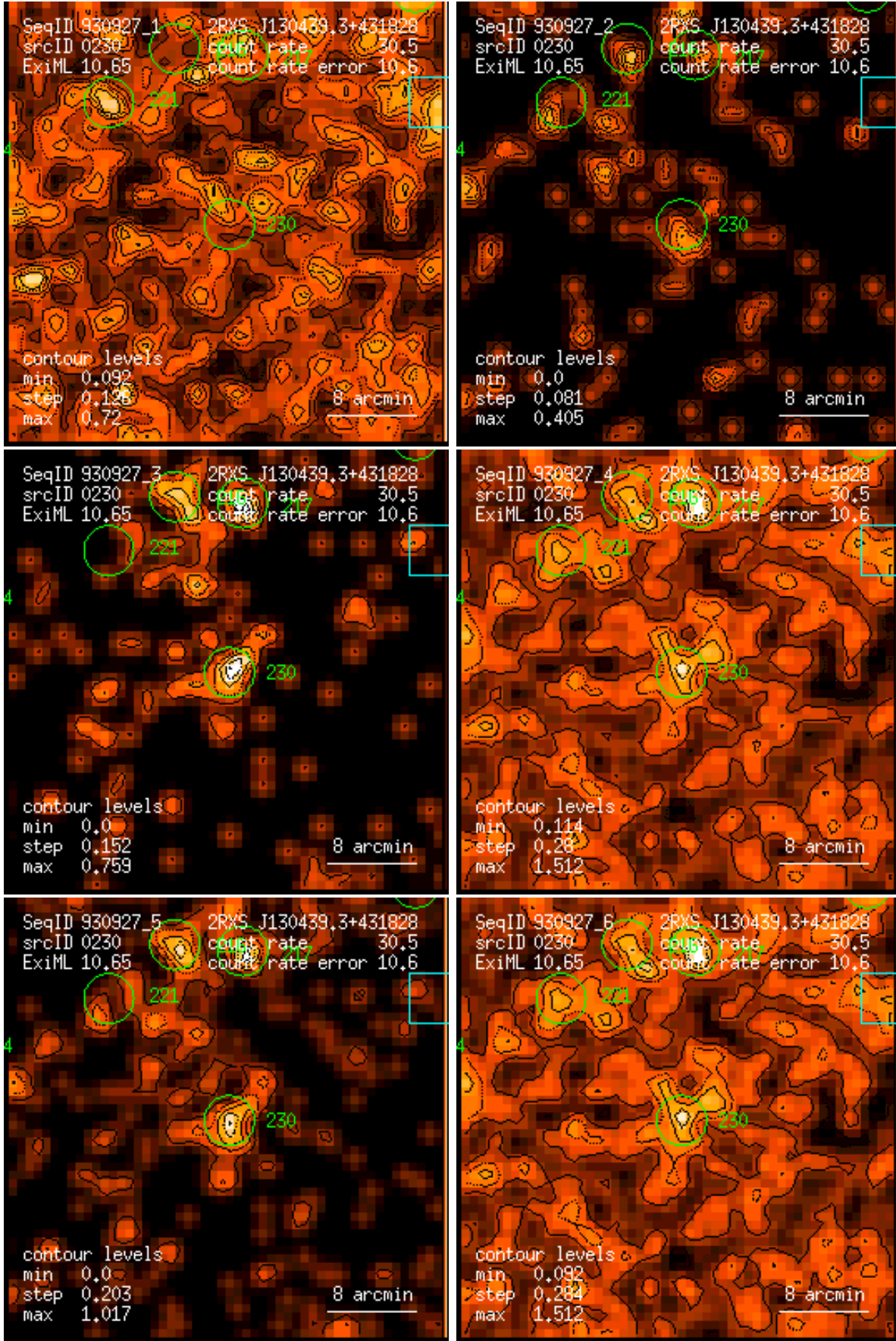
Figure 230: RASS 930927: detection 0230: band rate images, Gaussian filter: (1) PSPC channels 11 – 41, (2) 52 – 90, (3) 91 – 201, (4) 11 – 235, (5) 52 – 201, (6) 11 – 201. Broad band rates in counts/ks. Band rate contour levels in counts/ks/arcmin 2 .
