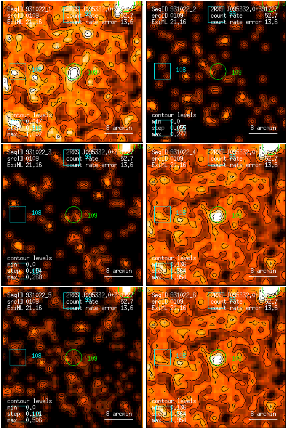
Figure 109: RASS 931022: detection 0109: band rate images, Gaussian filter: (1) PSPC channels 11 – 41, (2) 52 – 90, (3) 91 – 201, (4) 11 – 235, (5) 52 – 201, (6) 11 – 201. Broad band rates in counts/ks. Band rate contour levels in counts/ks/arcmin 2 .
