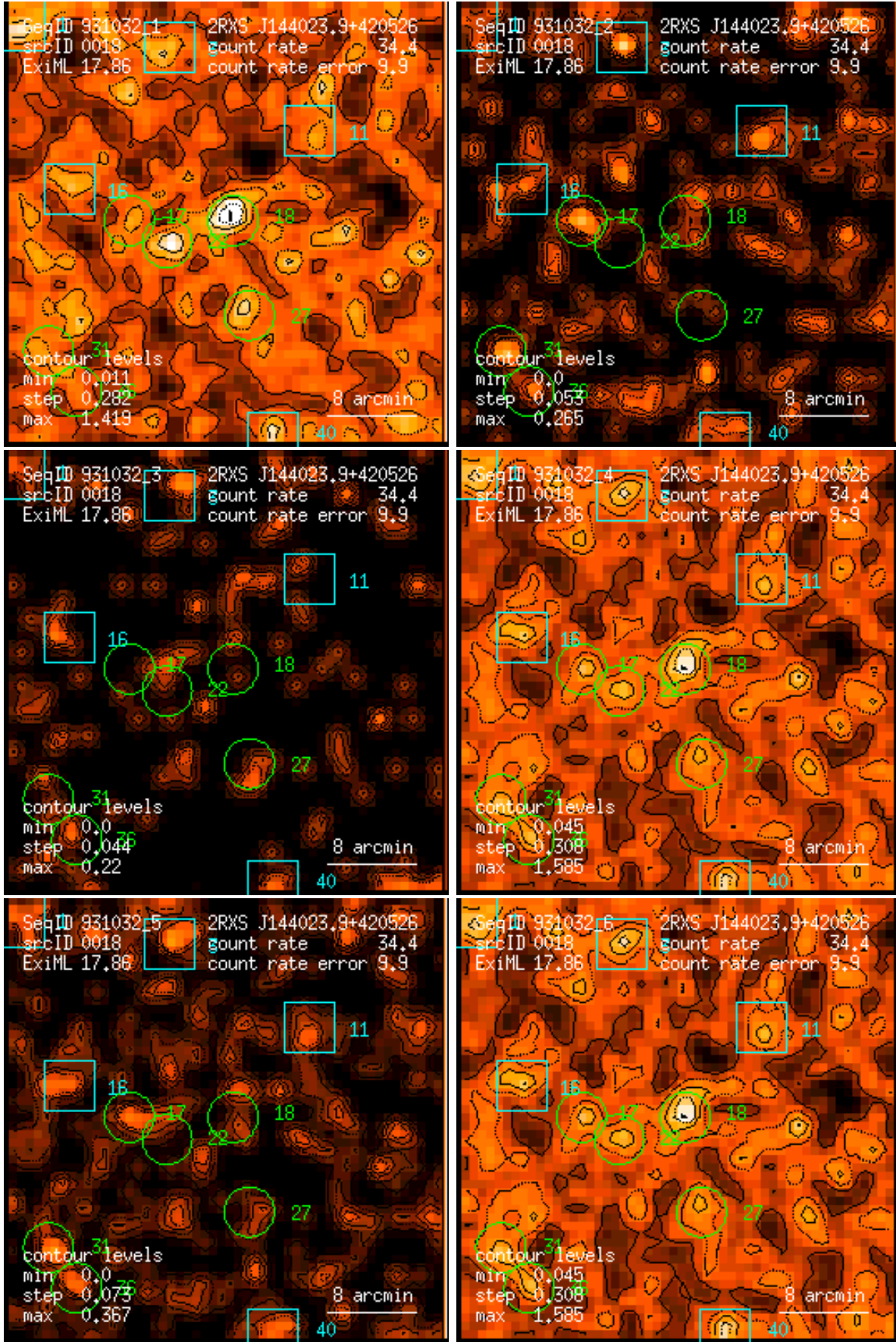
Figure 18: RASS 931032: detection 0018: band rate images, Gaussian filter: (1) PSPC channels 11 – 41, (2) 52 – 90, (3) 91 – 201, (4) 11 – 235, (5) 52 – 201, (6) 11 – 201. Broad band rates in counts/ks. Band rate contour levels in counts/ks/arcmin 2 .
