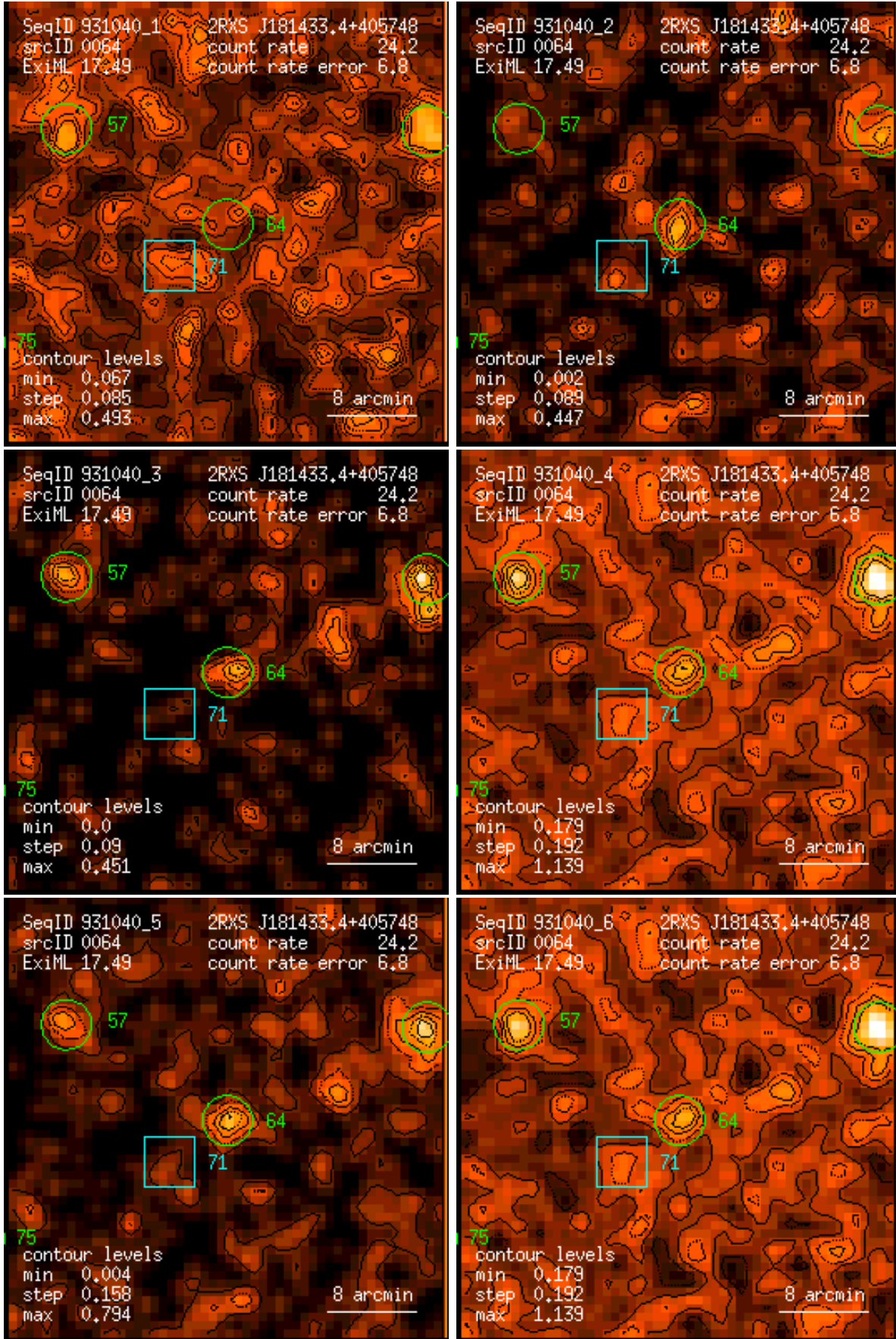
Figure 64: RASS 931040: detection 0064: band rate images, Gaussian filter: (1) PSPC channels 11 – 41, (2) 52 – 90, (3) 91 – 201, (4) 11 – 235, (5) 52 – 201, (6) 11 – 201. Broad band rates in counts/ks. Band rate contour levels in counts/ks/arcmin 2 .
