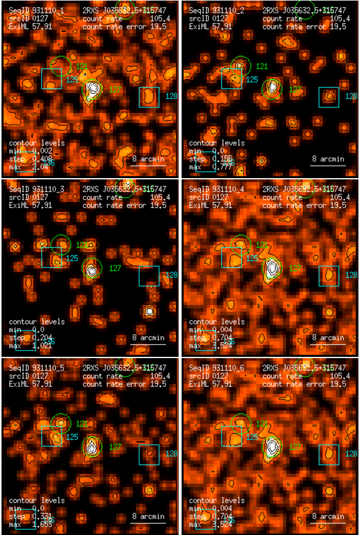
Figure 127: RASS 931110: detection 0127: band rate images, Gaussian filter: (1) PSPC channels 11 – 41, (2) 52 – 90, (3) 91 – 201, (4) 11 – 235, (5) 52 – 201, (6) 11 – 201. Broad band rates in counts/ks. Band rate contour levels in counts/ks/arcmin 2 .
