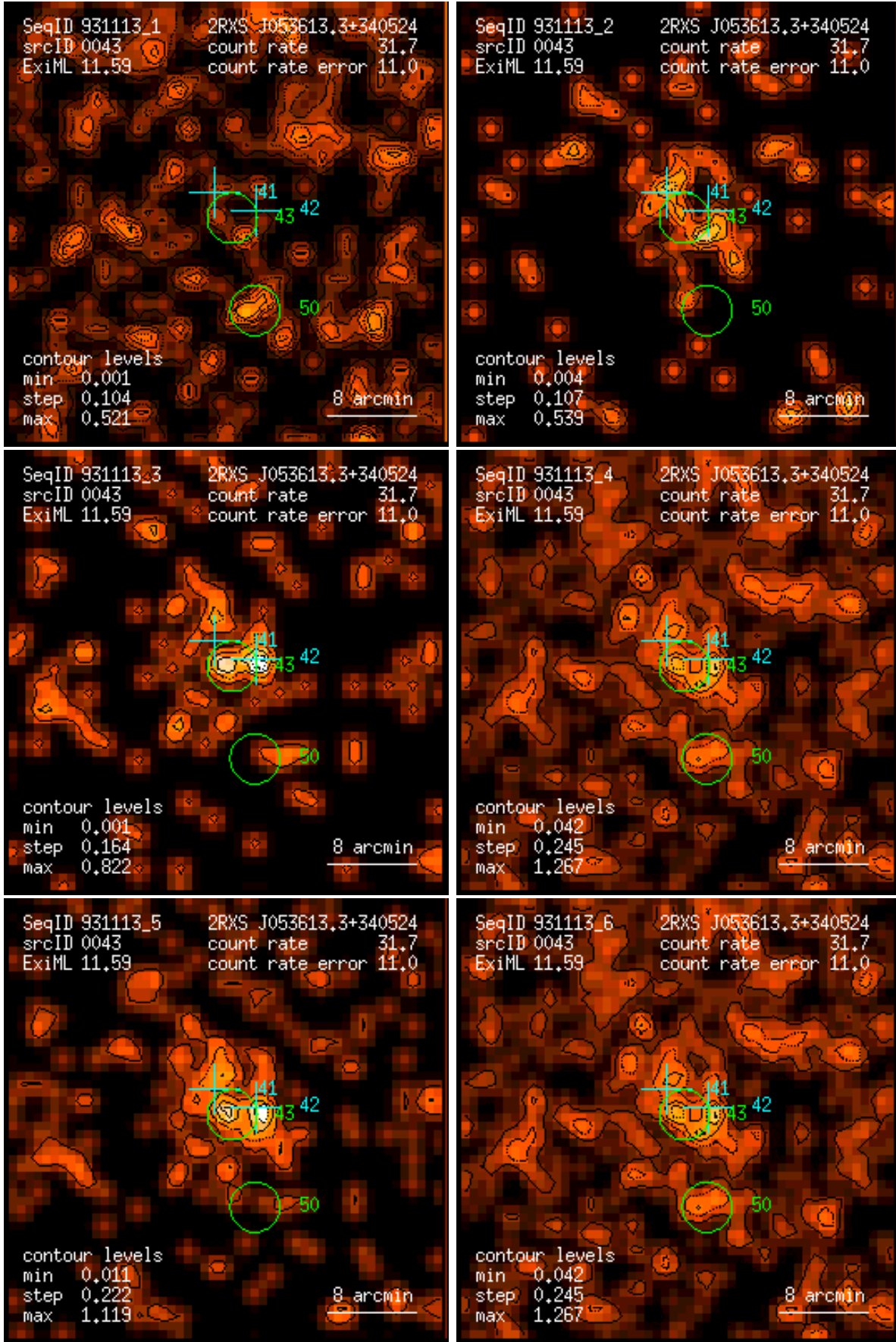
Figure 43: RASS 931113: detection 0043: band rate images, Gaussian filter: (1) PSPC channels 11 – 41, (2) 52 – 90, (3) 91 – 201, (4) 11 – 235, (5) 52 – 201, (6) 11 – 201. Broad band rates in counts/ks. Band rate contour levels in counts/ks/arcmin 2 .
