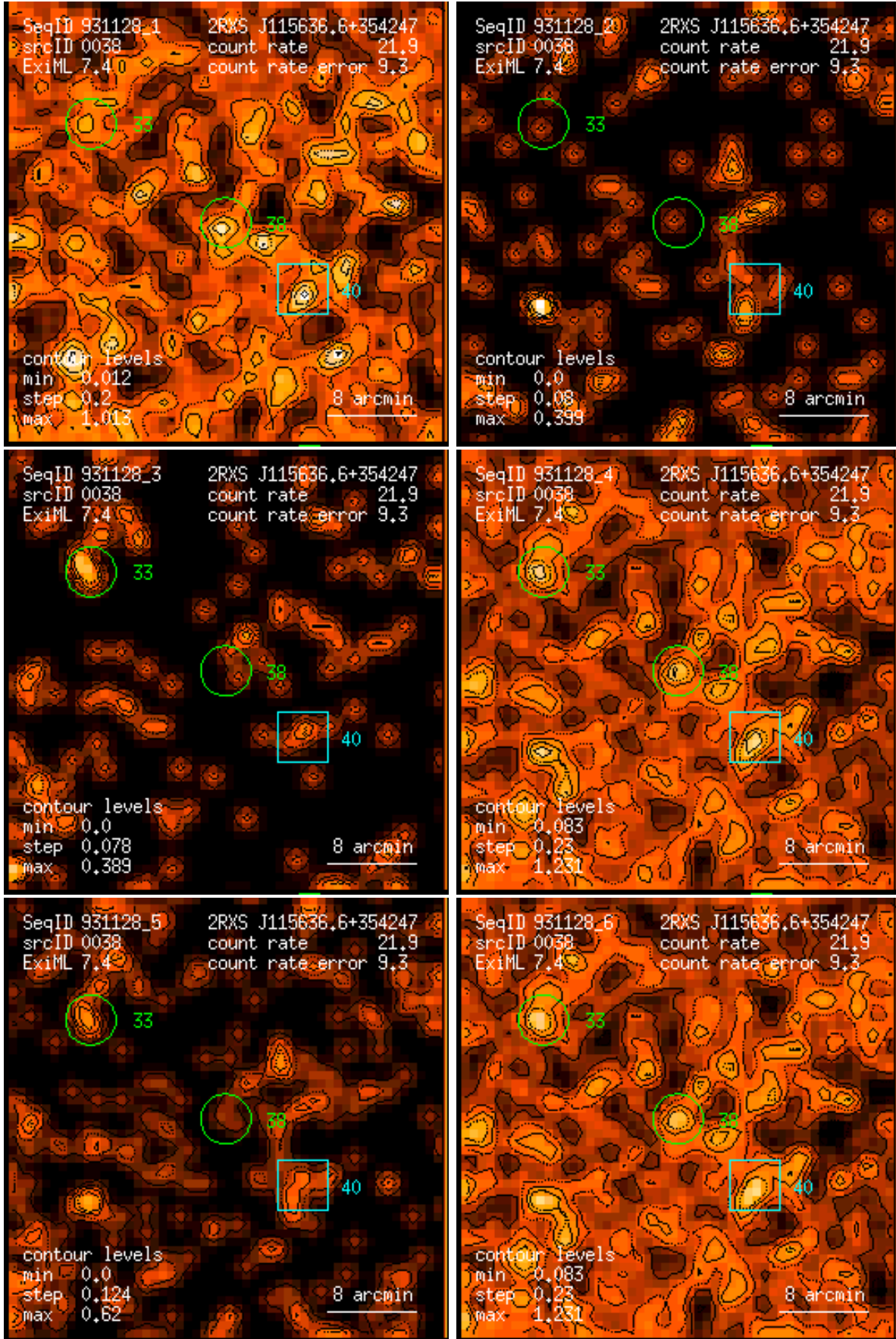
Figure 38: RASS 931128: detection 0038: band rate images, Gaussian filter: (1) PSPC channels 11 – 41, (2) 52 – 90, (3) 91 – 201, (4) 11 – 235, (5) 52 – 201, (6) 11 – 201. Broad band rates in counts/ks. Band rate contour levels in counts/ks/arcmin 2 .
