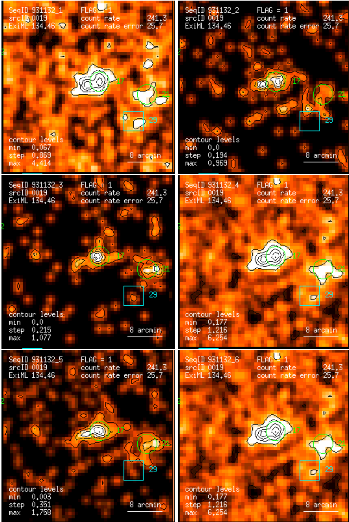
Figure 19: RASS 931132: detection 0019: band rate images, Gaussian filter: (1) PSPC channels 11 – 41, (2) 52 – 90, (3) 91 – 201, (4) 11 – 235, (5) 52 – 201, (6) 11 – 201. Broad band rates in counts/ks. Band rate contour levels in counts/ks/arcmin 2 .
