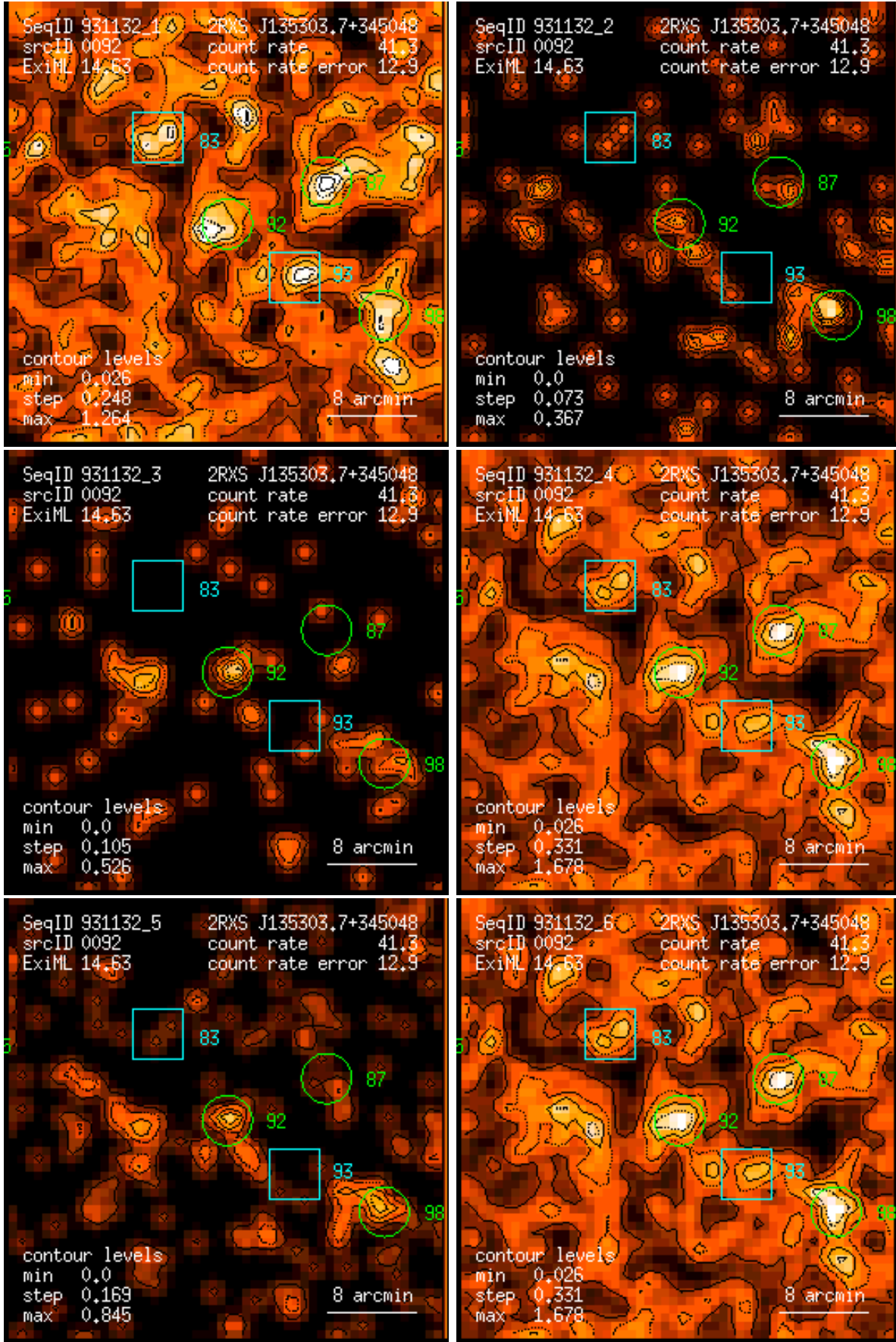
Figure 92: RASS 931132: detection 0092: band rate images, Gaussian filter: (1) PSPC channels 11 – 41, (2) 52 – 90, (3) 91 – 201, (4) 11 – 235, (5) 52 – 201, (6) 11 – 201. Broad band rates in counts/ks. Band rate contour levels in counts/ks/arcmin 2 .
