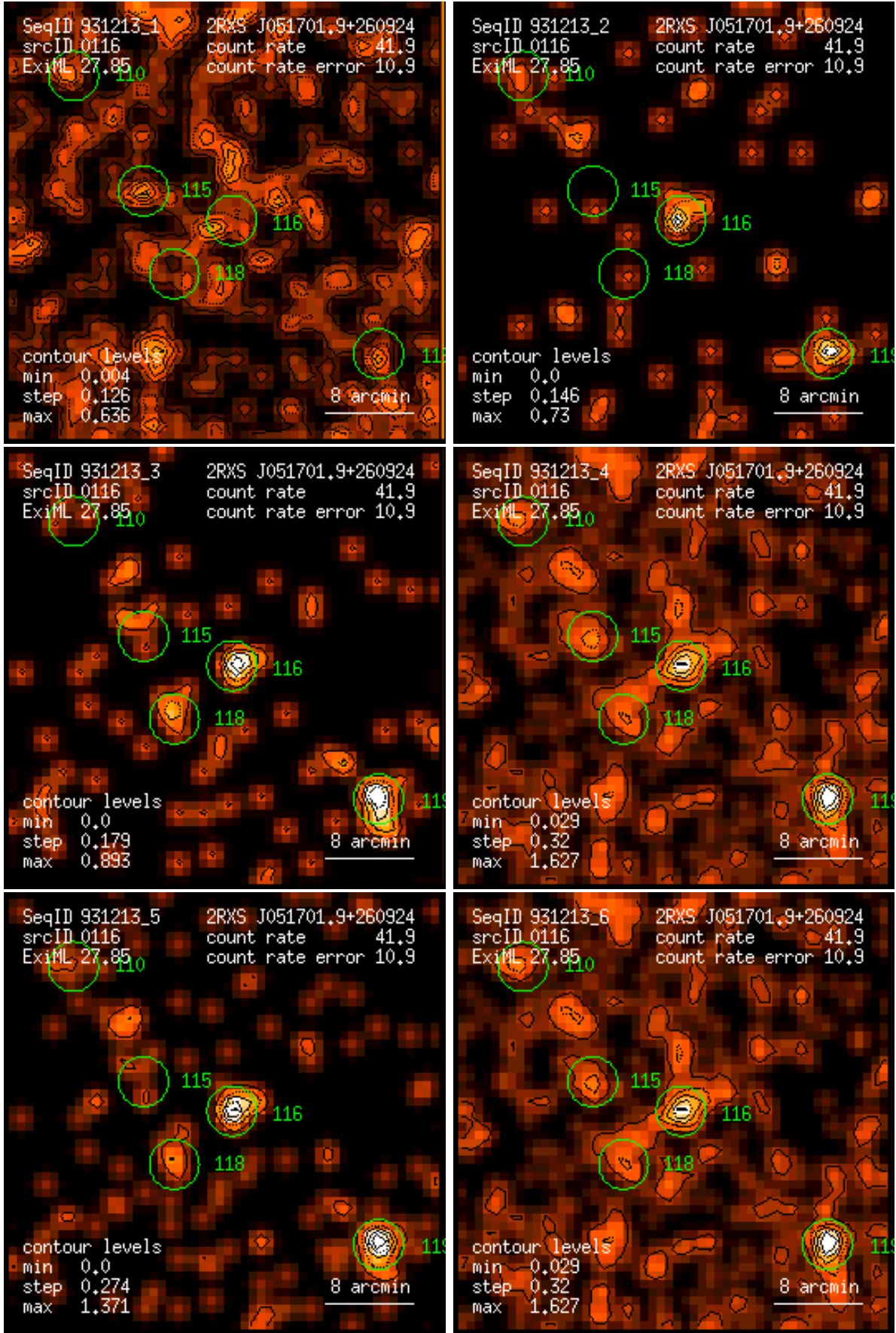
Figure 116: RASS 931213: detection 0116: band rate images, Gaussian filter: (1) PSPC channels 11 – 41, (2) 52 – 90, (3) 91 – 201, (4) 11 – 235, (5) 52 – 201, (6) 11 – 201. Broad band rates in counts/ks. Band rate contour levels in counts/ks/arcmin 2 .
