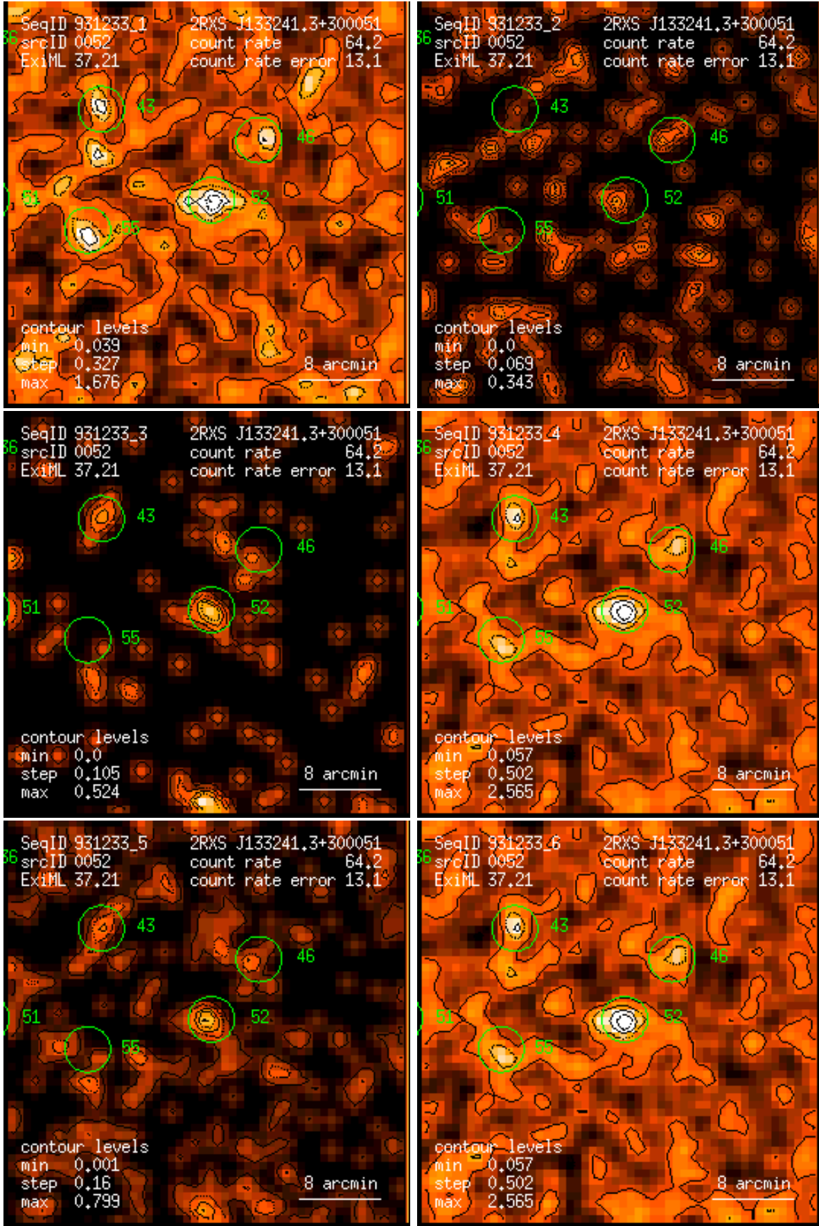
Figure 52: RASS 931233: detection 0052: band rate images, Gaussian filter: (1) PSPC channels 11 – 41, (2) 52 – 90, (3) 91 – 201, (4) 11 – 235, (5) 52 – 201, (6) 11 – 201. Broad band rates in counts/ks. Band rate contour levels in counts/ks/arcmin 2 .
