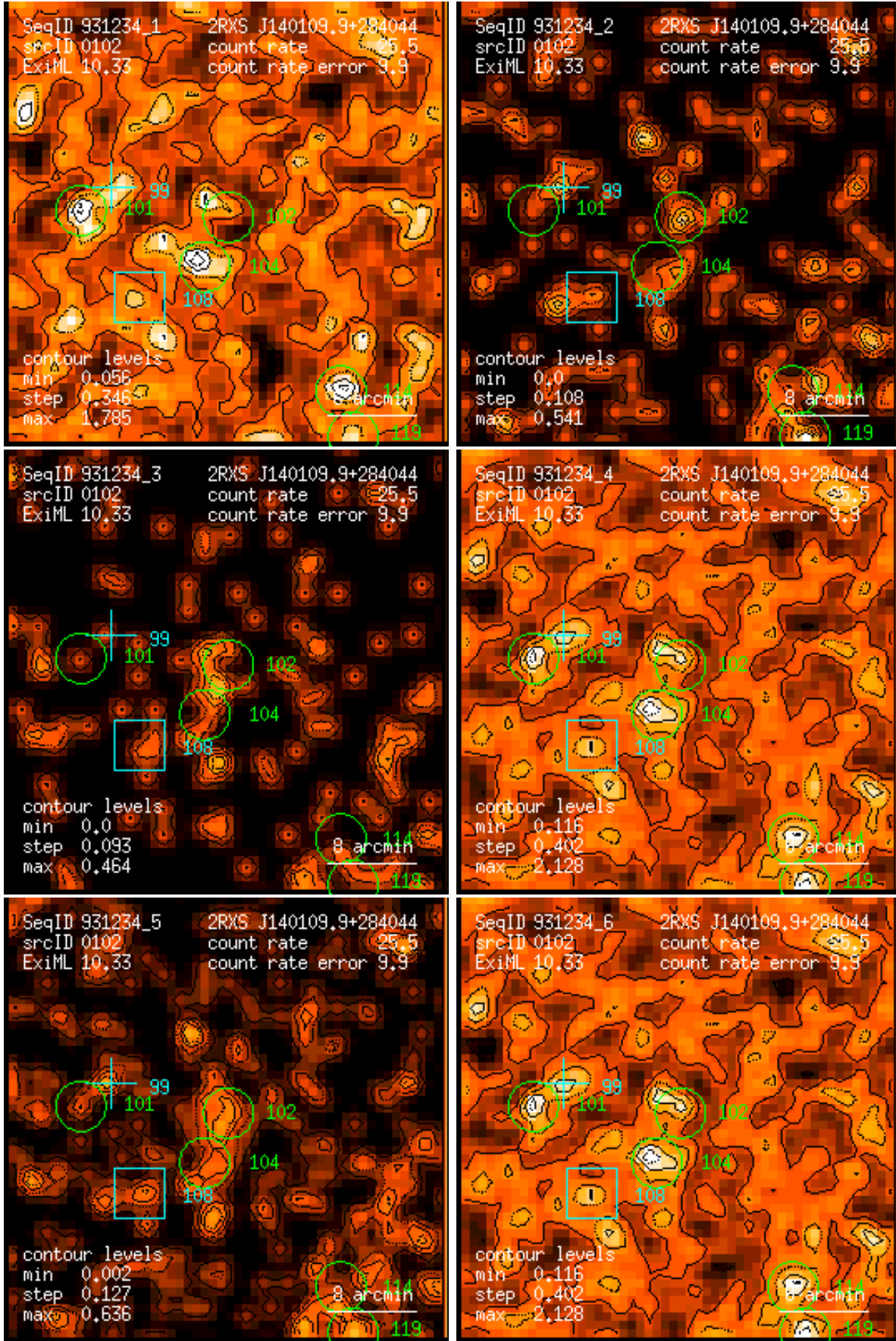
Figure 102: RASS 931234: detection 0102: band rate images, Gaussian filter: (1) PSPC channels 11 – 41, (2) 52 – 90, (3) 91 – 201, (4) 11 – 235, (5) 52 – 201, (6) 11 – 201. Broad band rates in counts/ks. Band rate contour levels in counts/ks/arcmin 2 .
