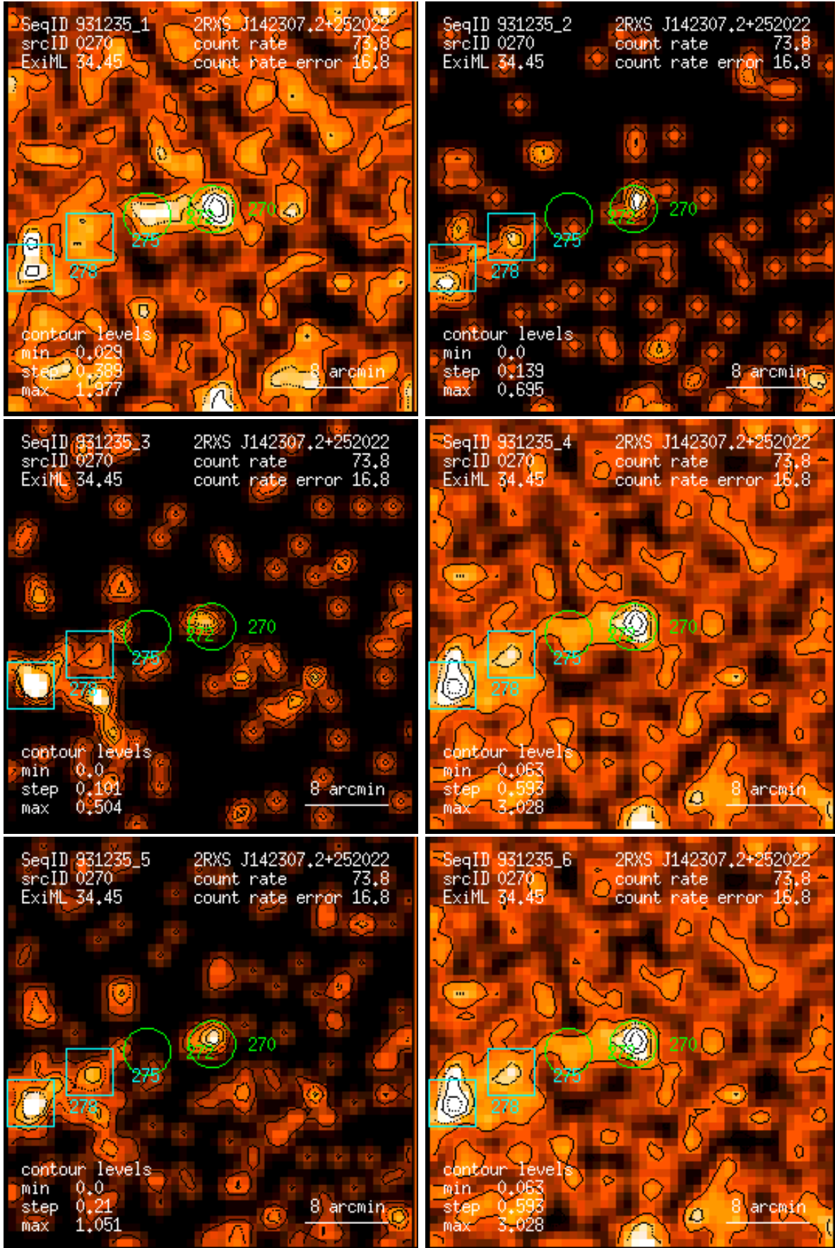
Figure 270: RASS 931235: detection 0270: band rate images, Gaussian filter: (1) PSPC channels 11 – 41, (2) 52 – 90, (3) 91 – 201, (4) 11 – 235, (5) 52 – 201, (6) 11 – 201. Broad band rates in counts/ks. Band rate contour levels in counts/ks/arcmin 2 .
