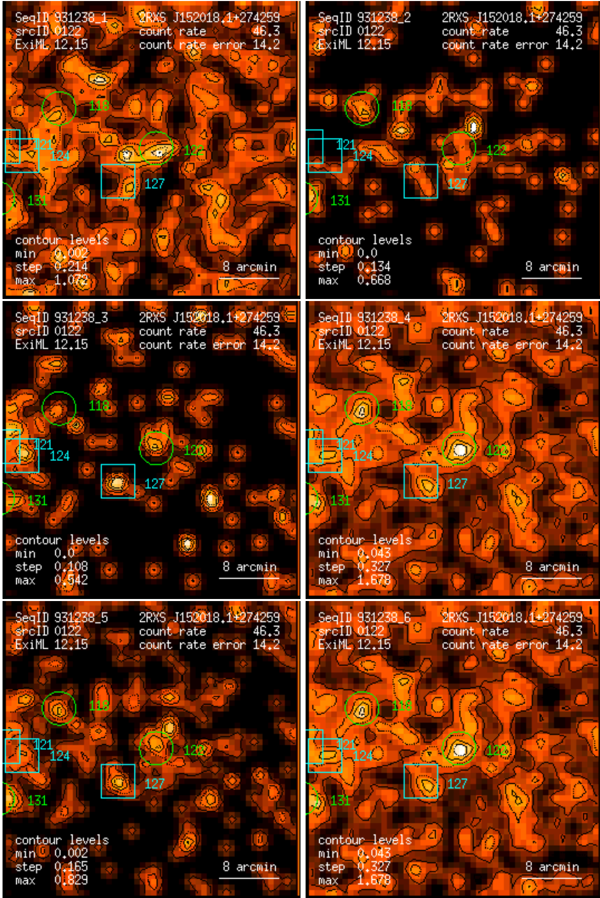
Figure 122: RASS 931238: detection 0122: band rate images, Gaussian filter: (1) PSPC channels 11 – 41, (2) 52 – 90, (3) 91 – 201, (4) 11 – 235, (5) 52 – 201, (6) 11 – 201. Broad band rates in counts/ks. Band rate contour levels in counts/ks/arcmin 2 .
