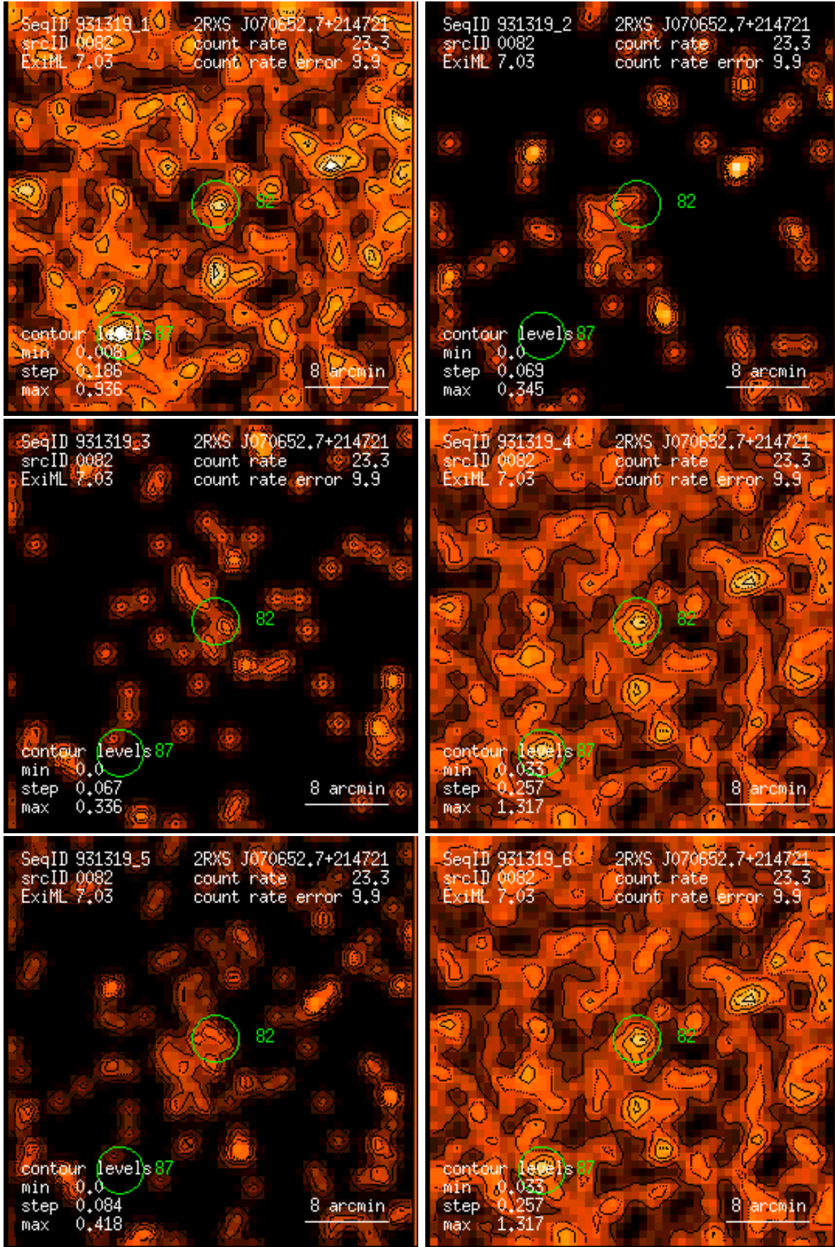
Figure 82: RASS 931319: detection 0082: band rate images, Gaussian filter: (1) PSPC channels 11 – 41, (2) 52 – 90, (3) 91 – 201, (4) 11 – 235, (5) 52 – 201, (6) 11 – 201. Broad band rates in counts/ks. Band rate contour levels in counts/ks/arcmin 2 .
