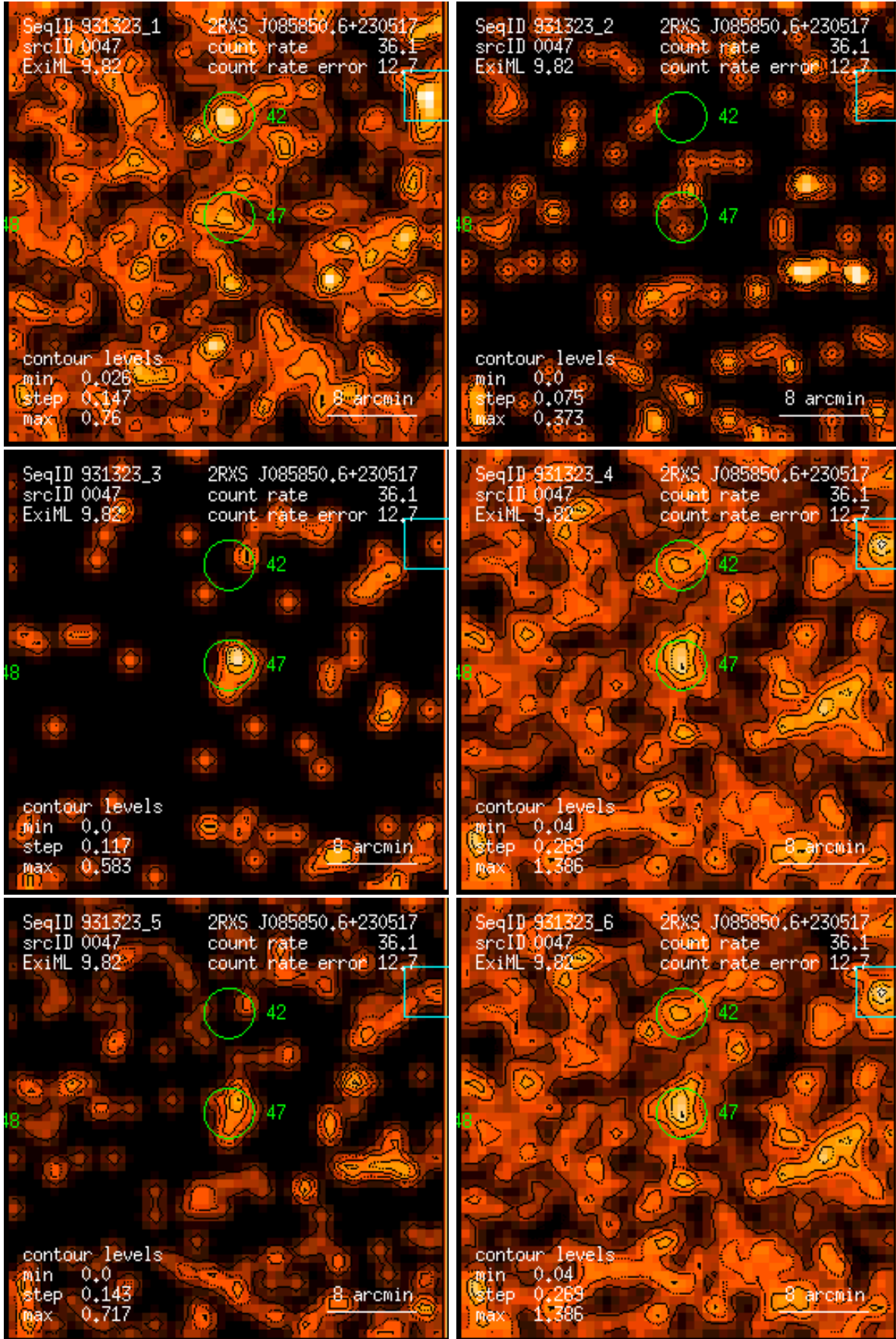
Figure 47: RASS 931323: detection 0047: band rate images, Gaussian filter: (1) PSPC channels 11 – 41, (2) 52 – 90, (3) 91 – 201, (4) 11 – 235, (5) 52 – 201, (6) 11 – 201. Broad band rates in counts/ks. Band rate contour levels in counts/ks/arcmin 2 .
