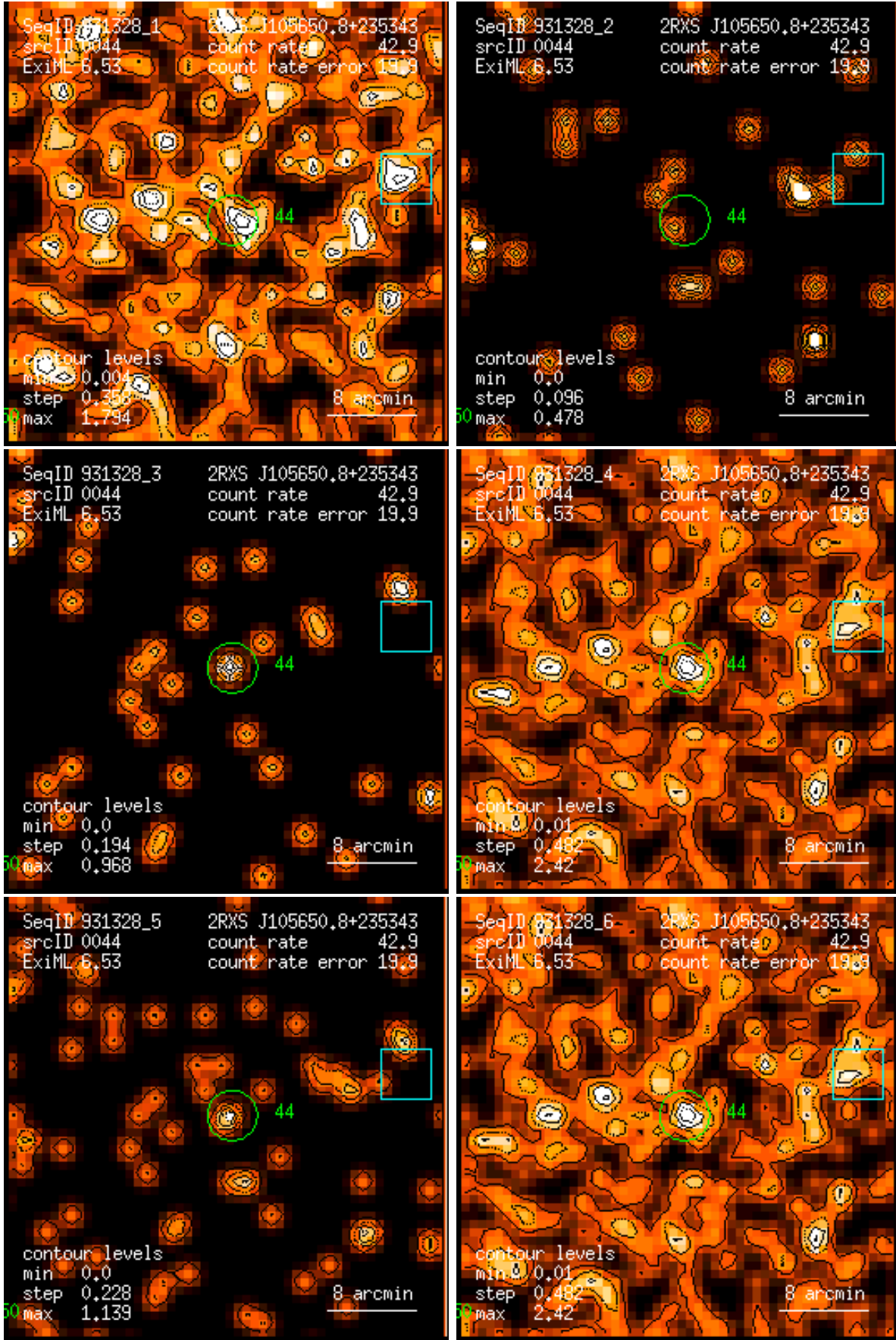
Figure 44: RASS 931328: detection 0044: band rate images, Gaussian filter: (1) PSPC channels 11 – 41, (2) 52 – 90, (3) 91 – 201, (4) 11 – 235, (5) 52 – 201, (6) 11 – 201. Broad band rates in counts/ks. Band rate contour levels in counts/ks/arcmin 2 .
