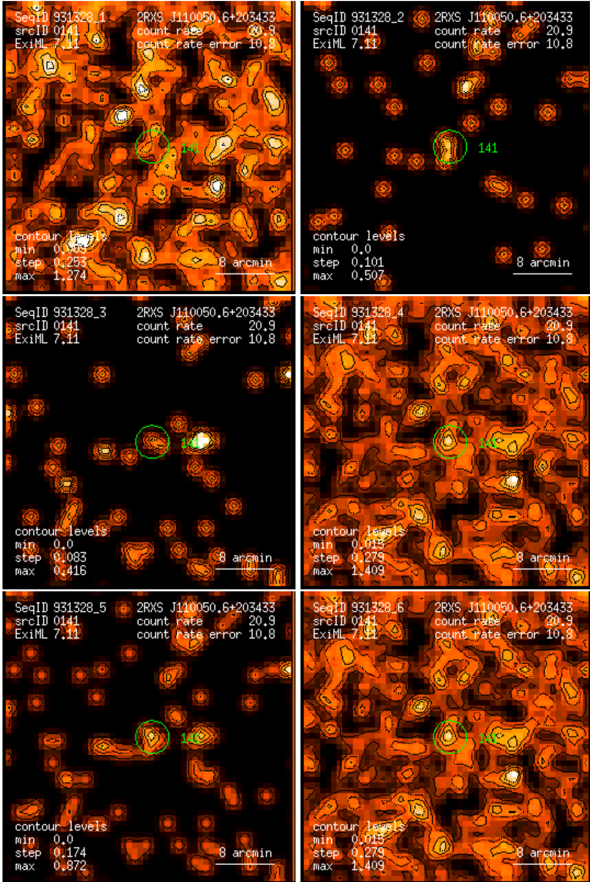
Figure 141: RASS 931328: detection 0141: band rate images, Gaussian filter: (1) PSPC channels 11 – 41, (2) 52 – 90, (3) 91 – 201, (4) 11 – 235, (5) 52 – 201, (6) 11 – 201. Broad band rates in counts/ks. Band rate contour levels in counts/ks/arcmin 2 .
