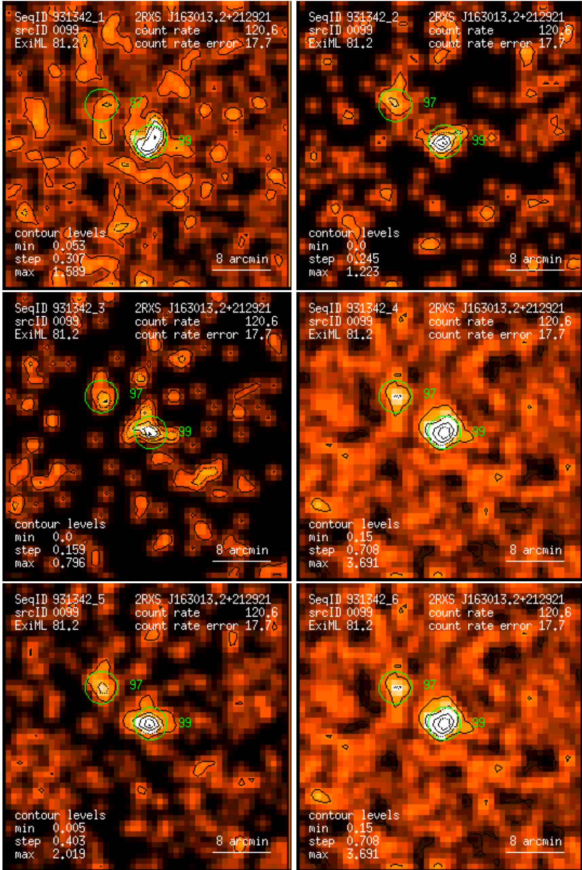
Figure 99: RASS 931342: detection 0099: band rate images, Gaussian filter: (1) PSPC channels 11 – 41, (2) 52 – 90, (3) 91 – 201, (4) 11 – 235, (5) 52 – 201, (6) 11 – 201. Broad band rates in counts/ks. Band rate contour levels in counts/ks/arcmin 2 .
