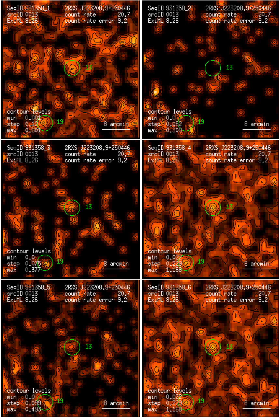
Figure 13: RASS 931358: detection 0013: band rate images, Gaussian filter: (1) PSPC channels 11 – 41, (2) 52 – 90, (3) 91 – 201, (4) 11 – 235, (5) 52 – 201, (6) 11 – 201. Broad band rates in counts/ks. Band rate contour levels in counts/ks/arcmin 2 .
