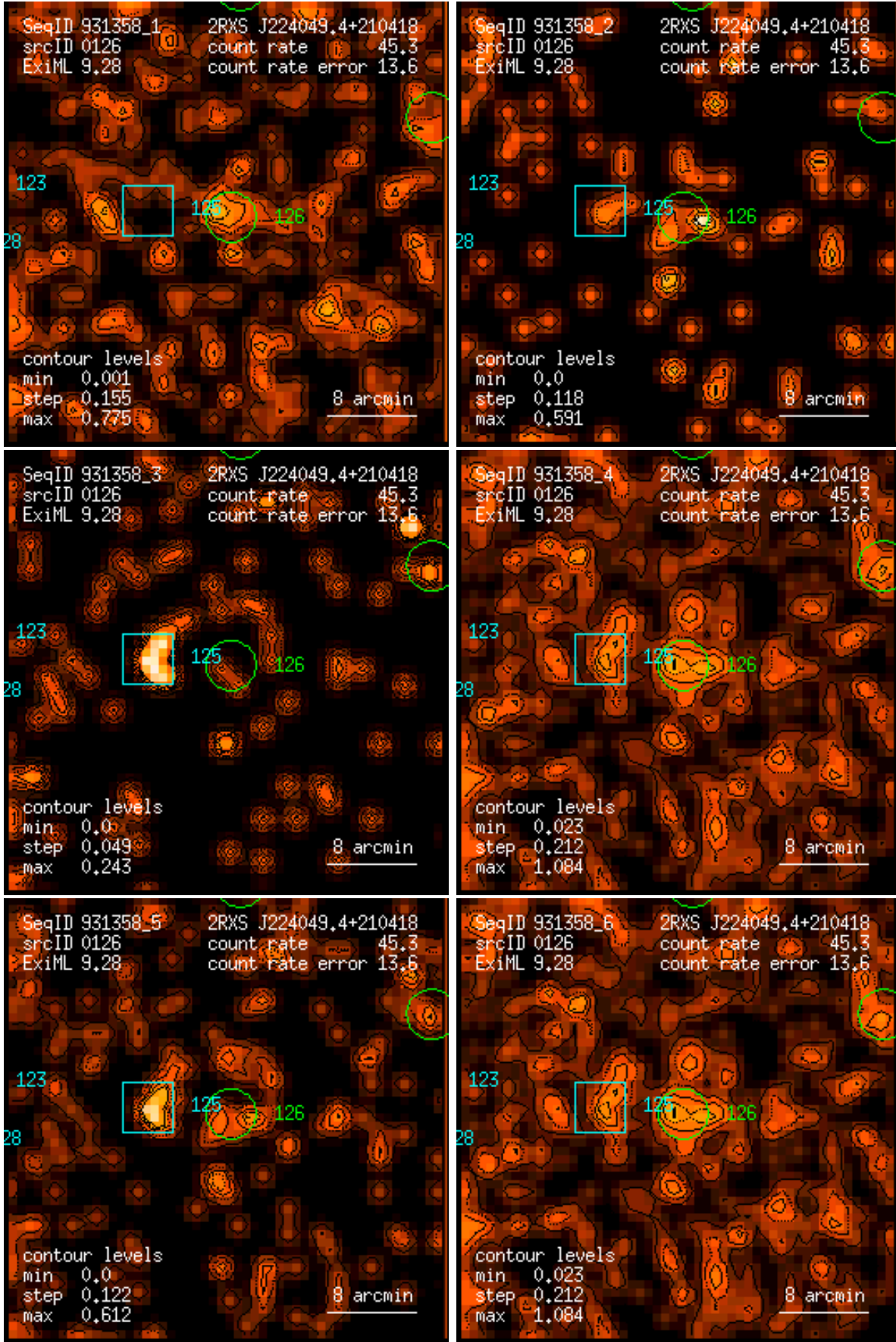
Figure 126: RASS 931358: detection 0126: band rate images, Gaussian filter: (1) PSPC channels 11 – 41, (2) 52 – 90, (3) 91 – 201, (4) 11 – 235, (5) 52 – 201, (6) 11 – 201. Broad band rates in counts/ks. Band rate contour levels in counts/ks/arcmin 2 .
