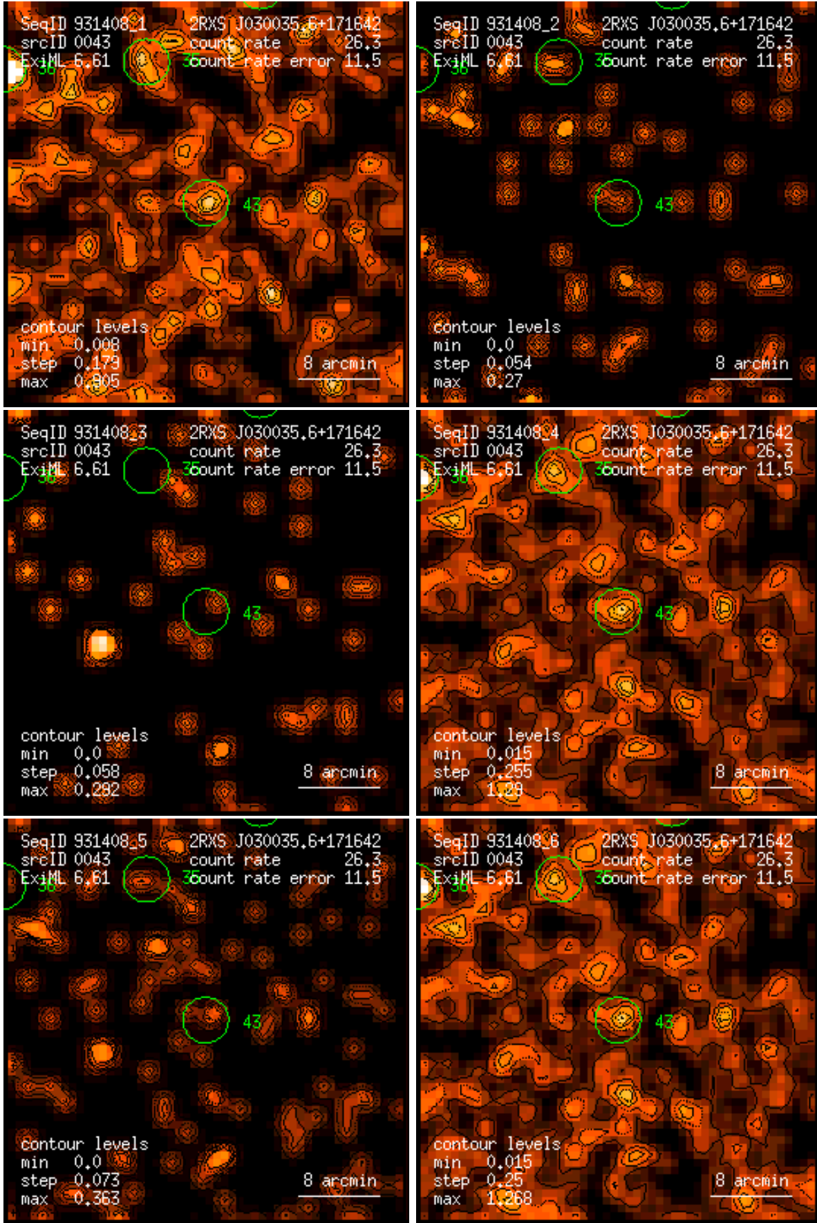
Figure 43: RASS 931408: detection 0043: band rate images, Gaussian filter: (1) PSPC channels 11 – 41, (2) 52 – 90, (3) 91 – 201, (4) 11 – 235, (5) 52 – 201, (6) 11 – 201. Broad band rates in counts/ks. Band rate contour levels in counts/ks/arcmin 2 .
