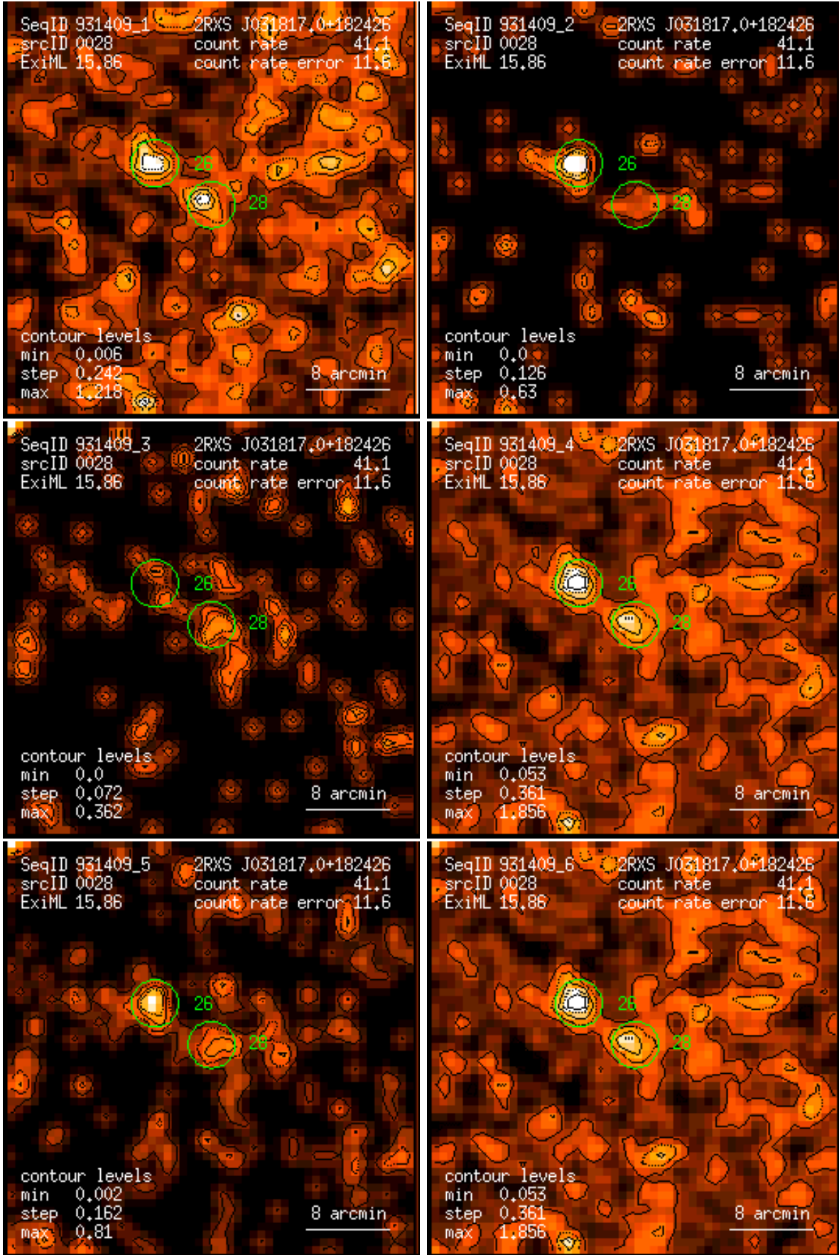
Figure 28: RASS 931409: detection 0028: band rate images, Gaussian filter: (1) PSPC channels 11 – 41, (2) 52 – 90, (3) 91 – 201, (4) 11 – 235, (5) 52 – 201, (6) 11 – 201. Broad band rates in counts/ks. Band rate contour levels in counts/ks/arcmin 2 .
